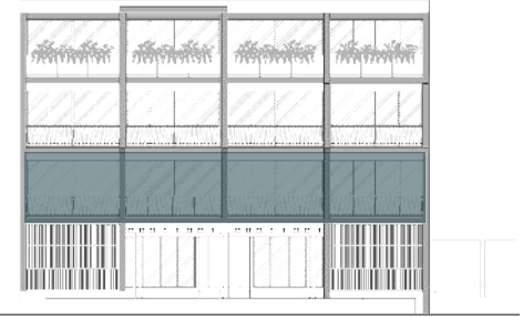
Facade Exterior - 85m
