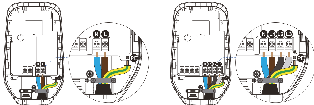
1P+N+PE
