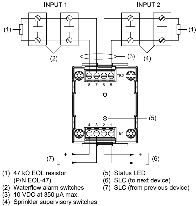
Figure 2: Wiring diagram
