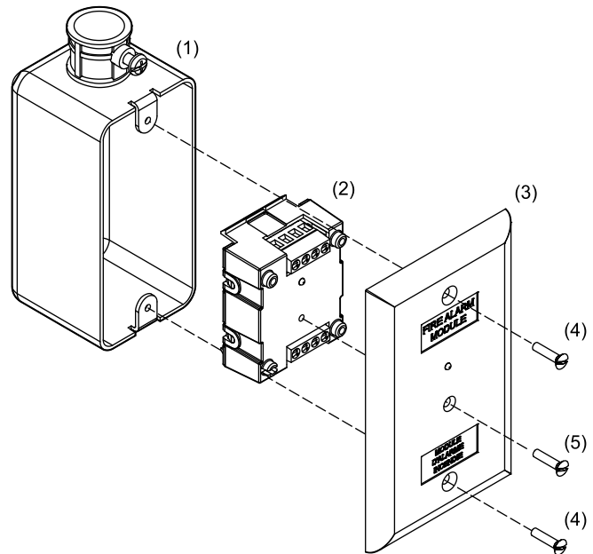
Figure 1: Installing the SIGA-WTM module
