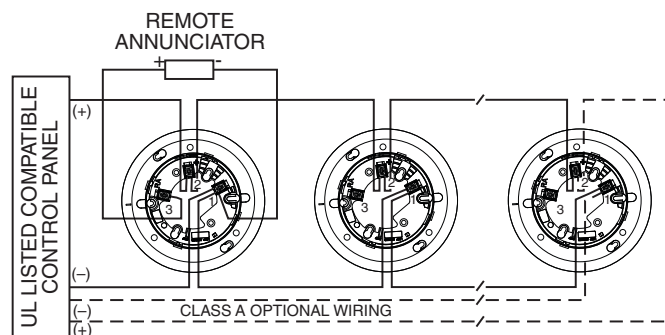
FIGURE 1. WIRING DIAGRAM
