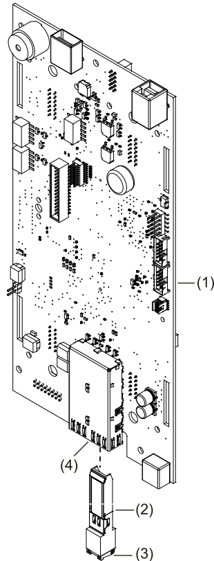
Figure 1: 4-NET-CAT installation
