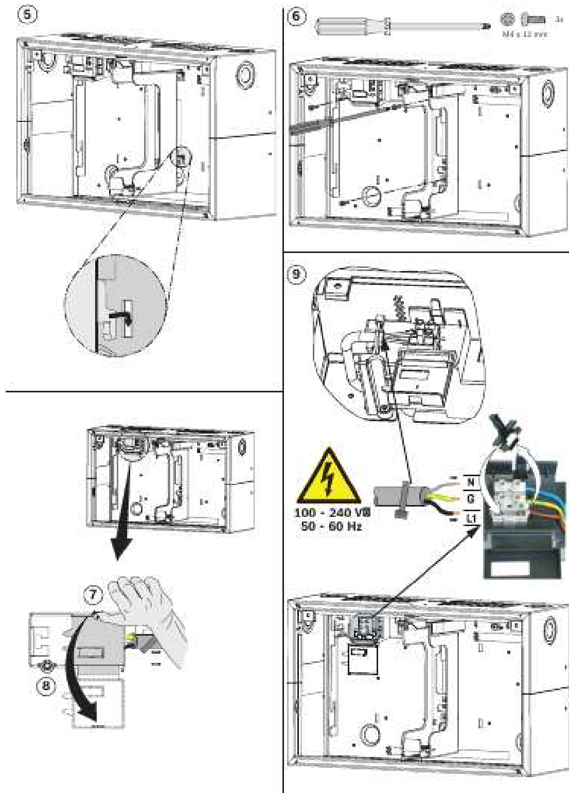
Figure 4.27: FPO-5000-PSB1 installation (5-9)
