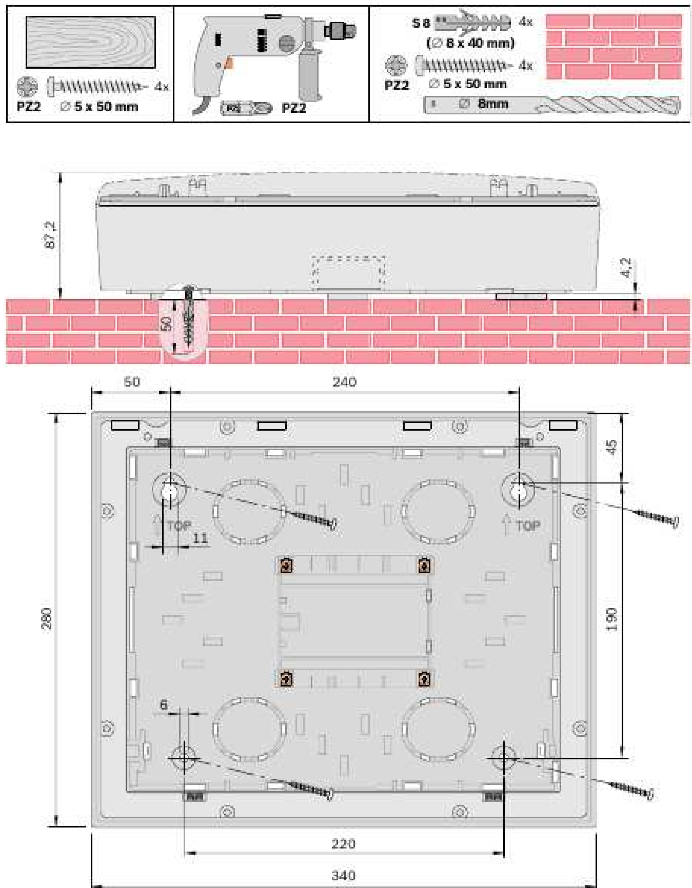
Figure 4.88: Remote Keypad surface mounting; dimensions in mm
