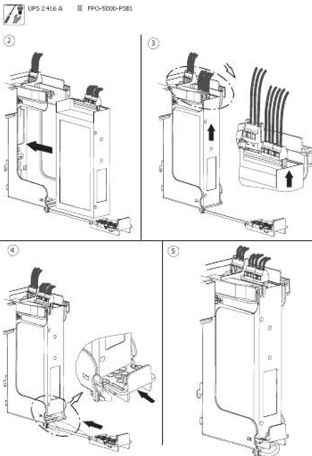
Figure 4.30: Installation of UPS 2416 A in FPO-5000-PSB1 (2-5)
