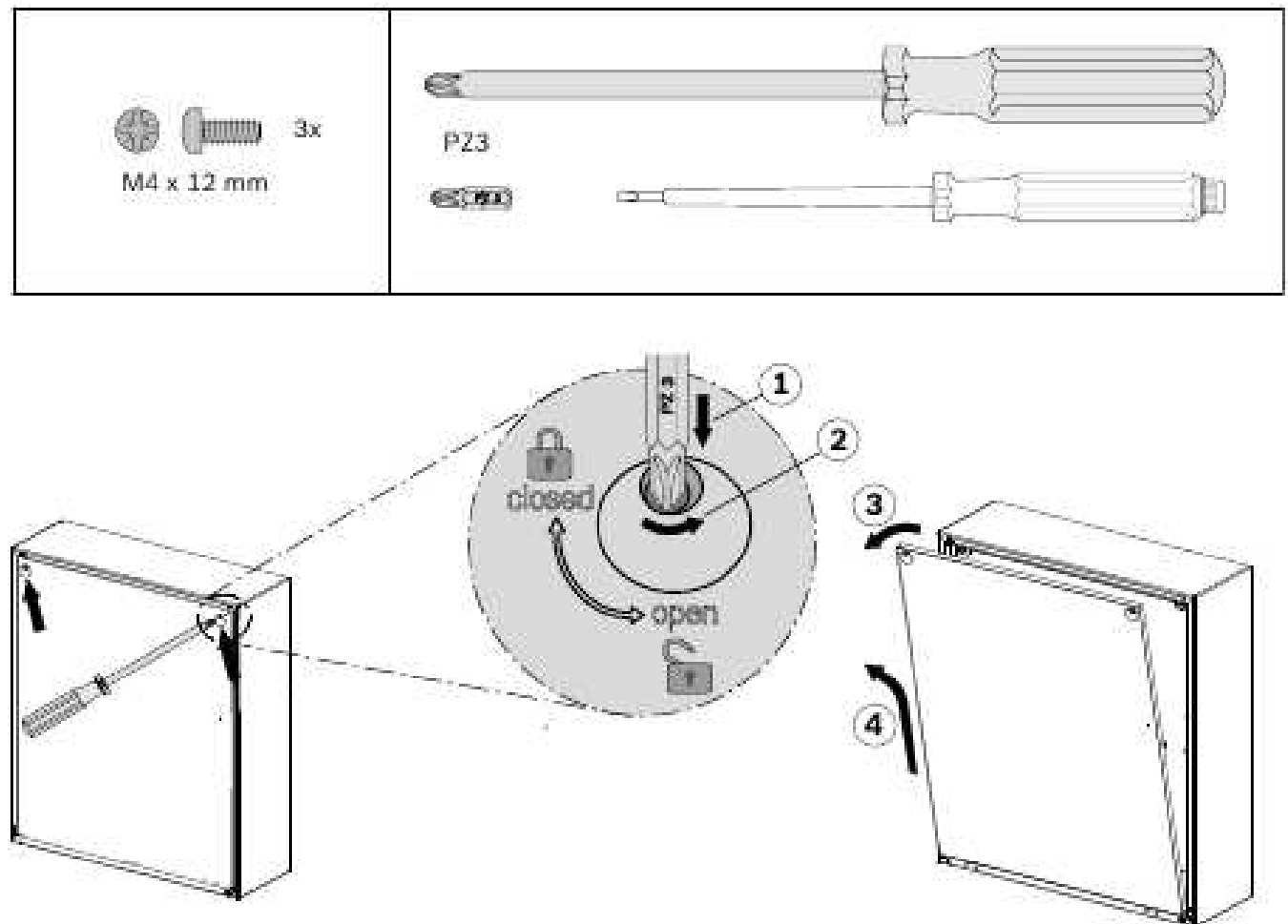
Figure 4.21: FPO-5000-PSB-CH/FPO-5000-PSB1 installation (1-4)
