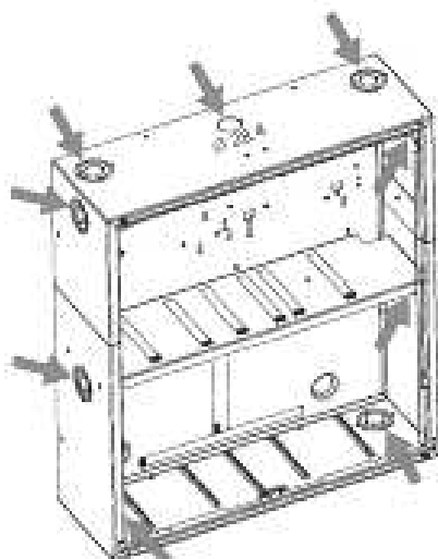
Figure 4.6: Wall mounting housing cable bushings
