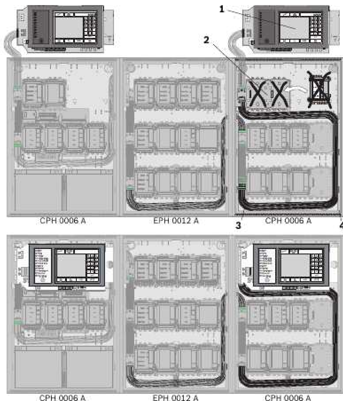
Figure 3.12: Redundant configuration
