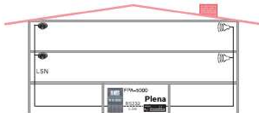
Figure 2.9: Connecting a Plena Voice Alarm System
