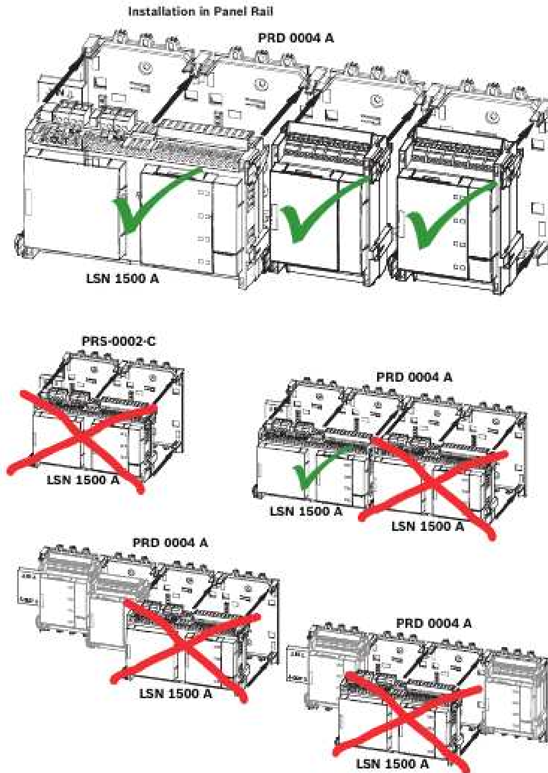
Figure 4.68: LSN 1500 A - Inserting the module
