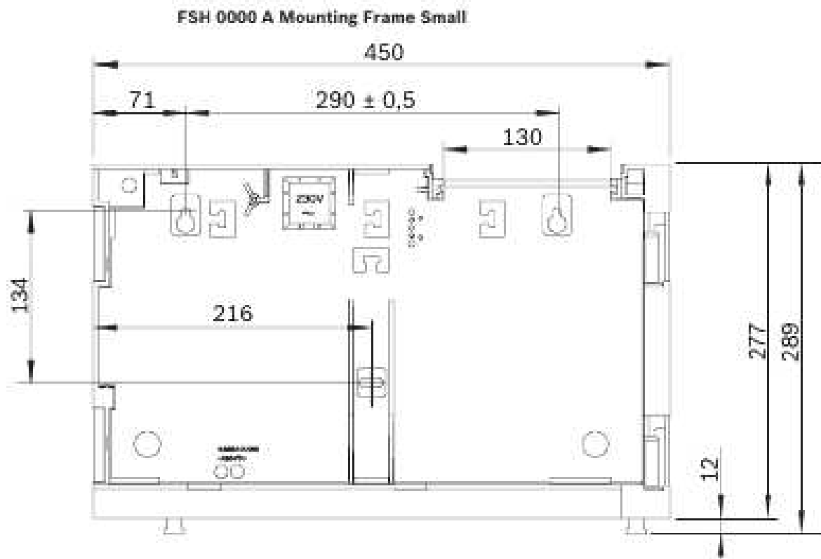
Figure 4.12: Installation dimensions - FSH 0000 A [in mm]
