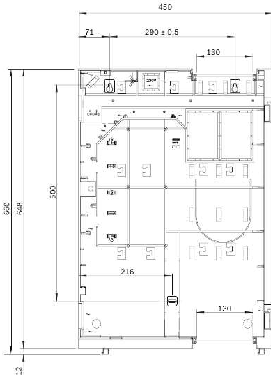
Figure 4.10: Mounting frame: Installation dimensions - FBH 0000 A/FHS 0000 A [in mm]
