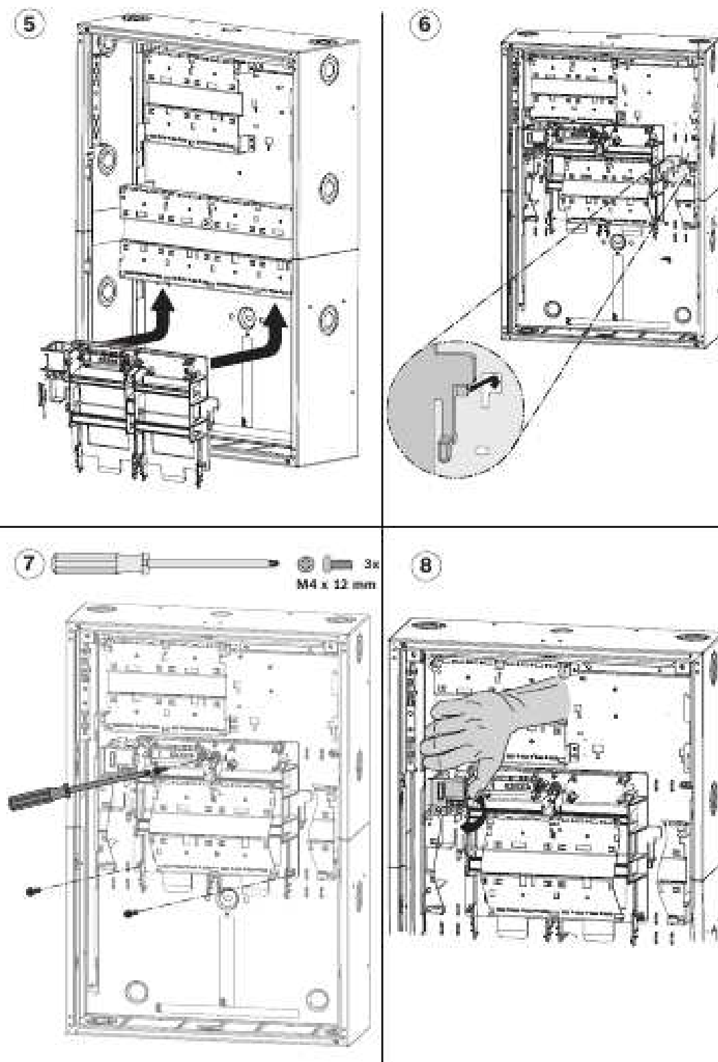
Figure 4.24: FPO-5000-PSB-CH installation (5-8)
