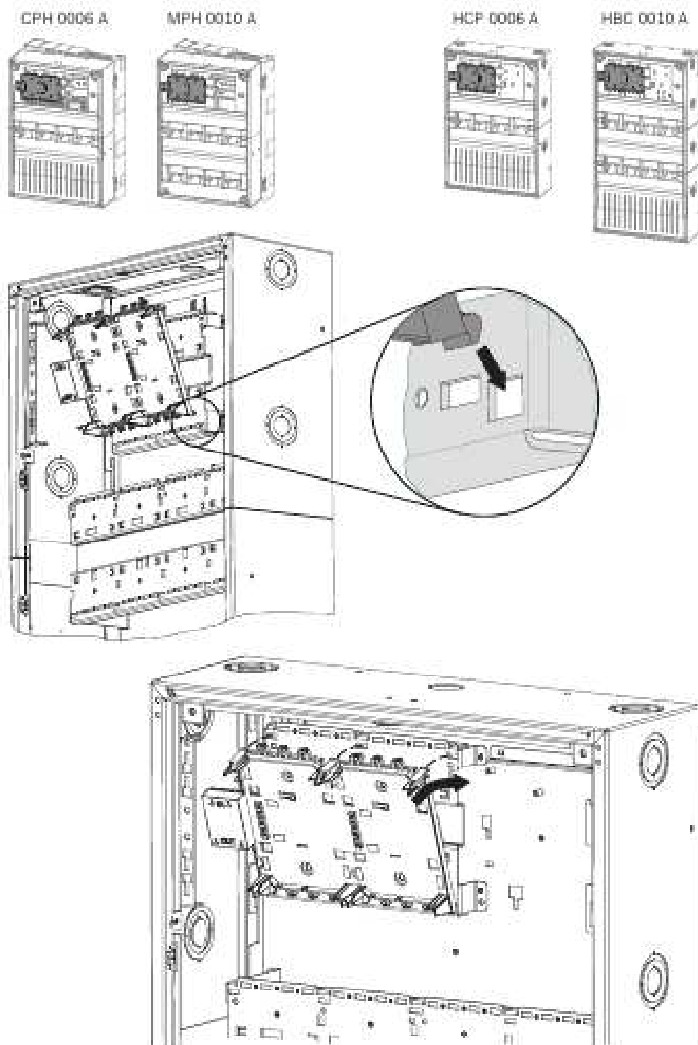
Figure 4.35: PRS-0002-C installation
