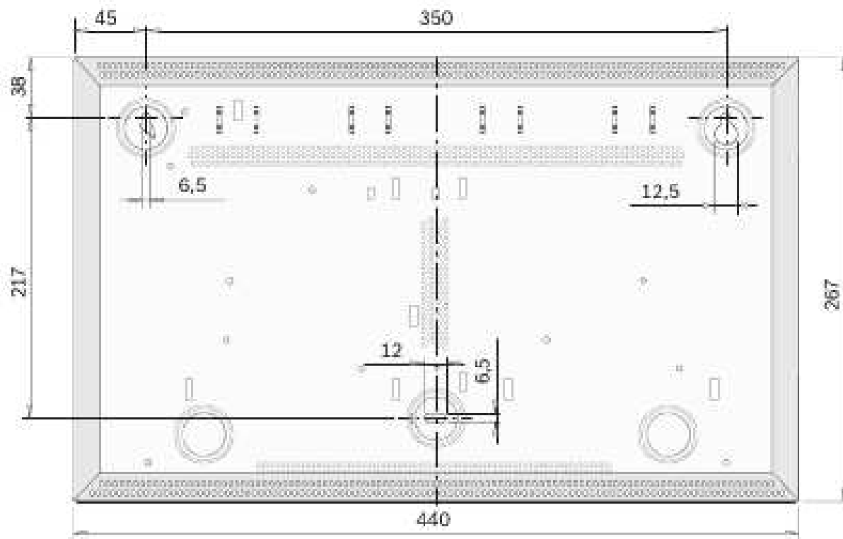
Figure 4.5: Installation dimensions - PSS 0002 A/DIB 0000 A [in mm]
