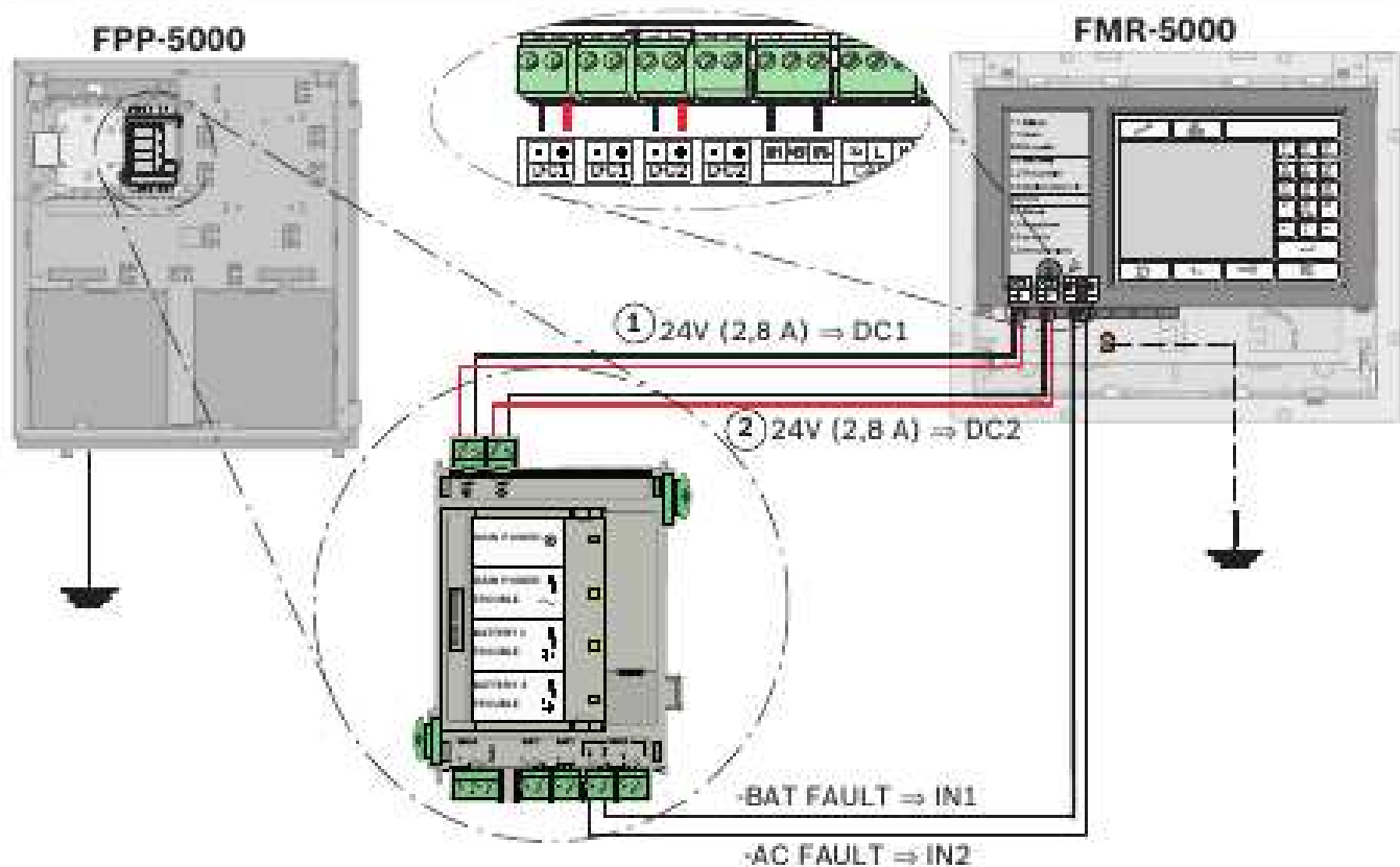
Figure 4.93: Remote Keypad wiring with BCM-0000-B
