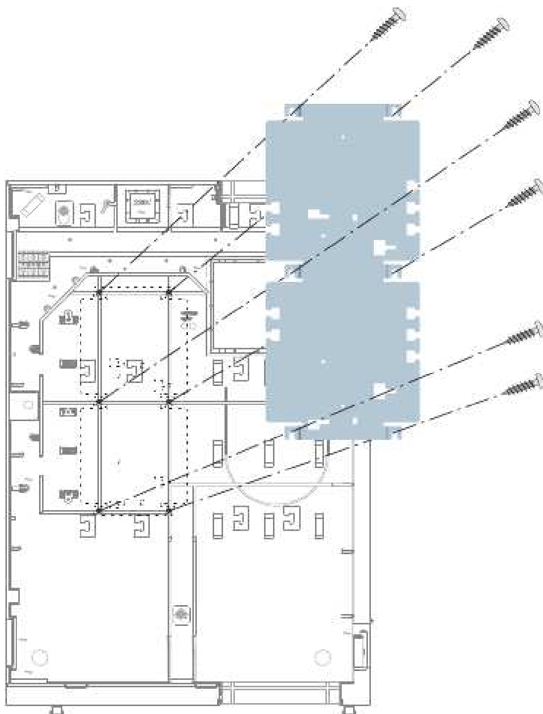
Figure 4.19: HMP 0003 A installation
