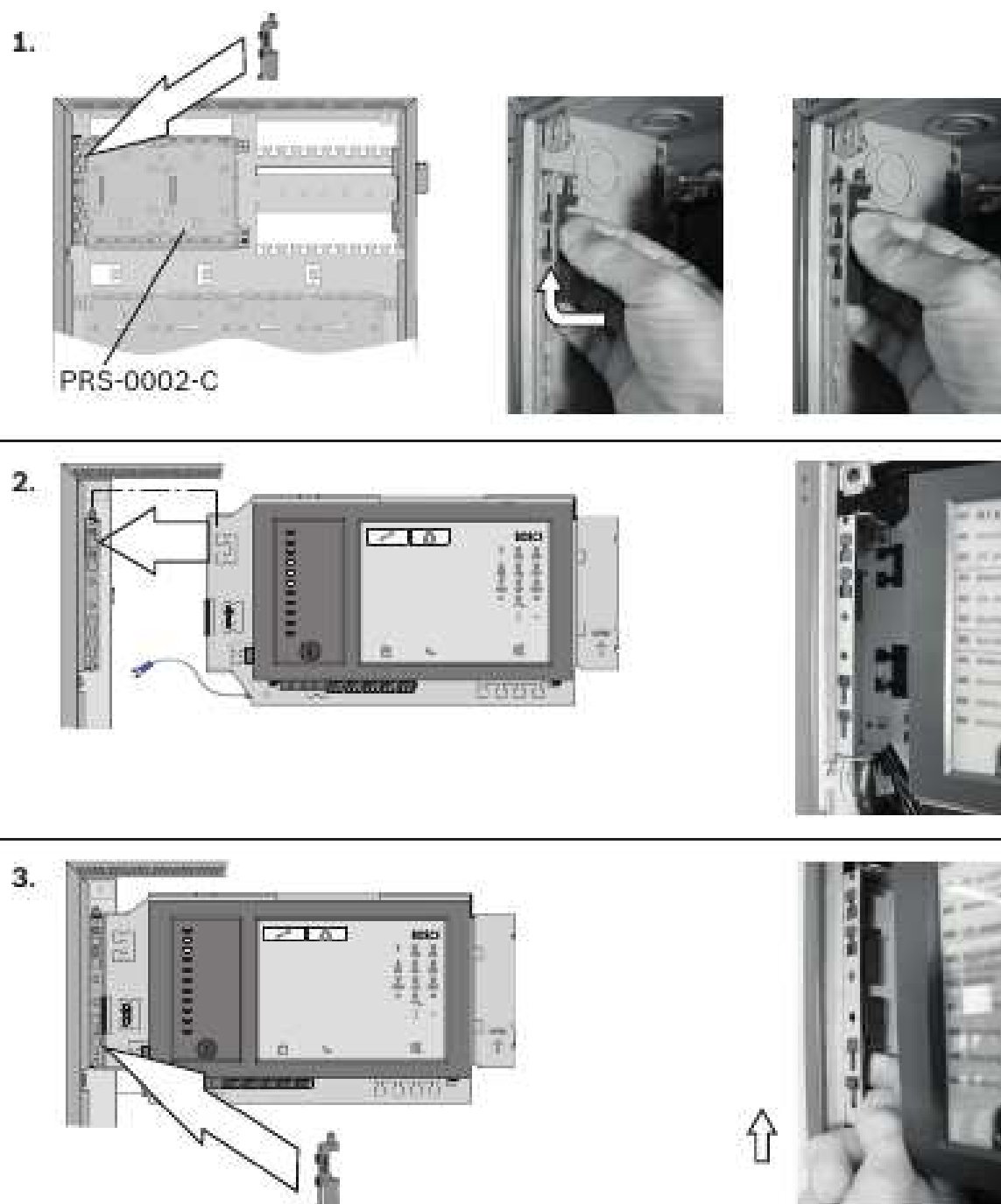
Figure 4.43: MPC installation (1-3)
