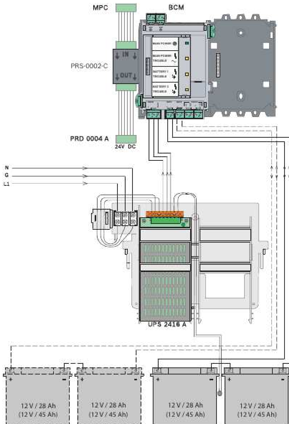
Figure 4.56: Wiring diagram for BCM-0000-B
