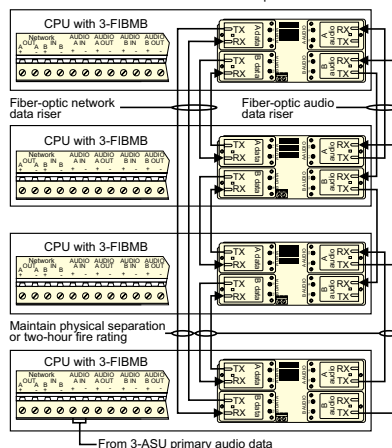
3-CPU Class X network and audio fiber-optic connections
