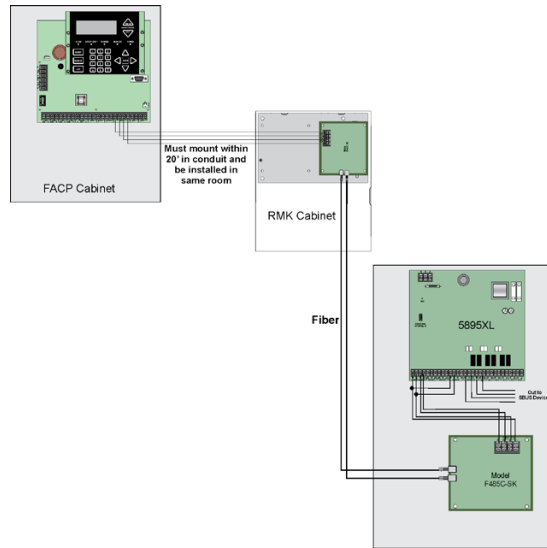
CONNECTING FIBER TO PANEL TO POWER SUPPLY
