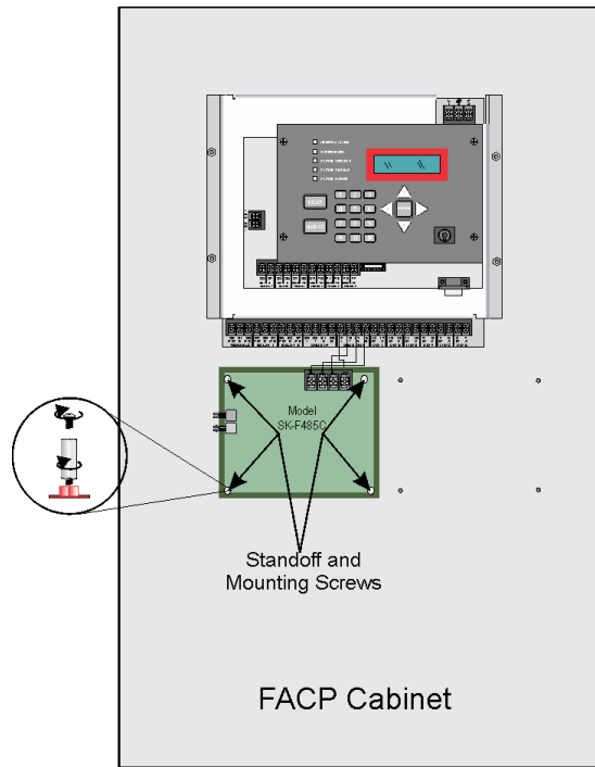
SK-F485C MOUNTING IN FACP CABINET
