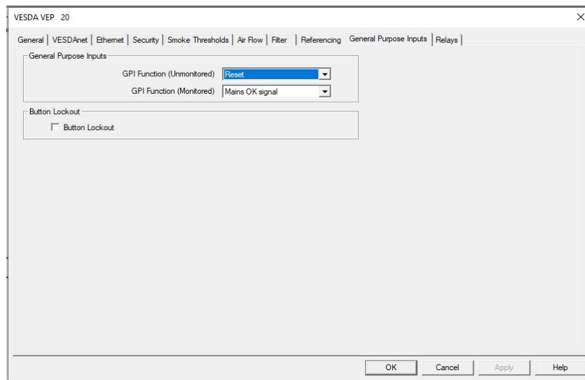
Figure 5-19: General Purpose Input Options
