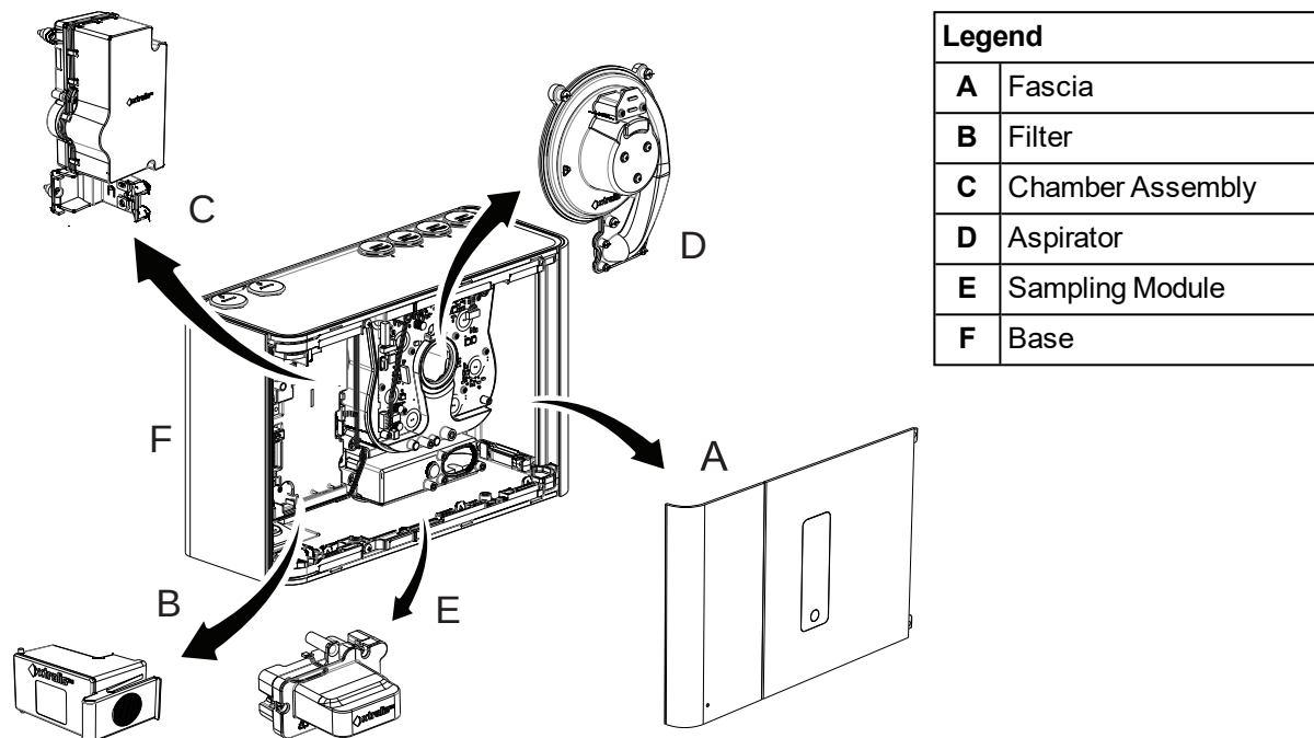
Figure 2-1: Detector components
