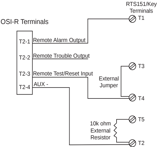
Figure 11-4: Wiring Diagram (RTS451 or RTS151)
