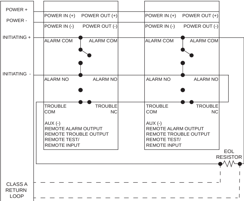
Figure 11-2: Wiring Diagram
