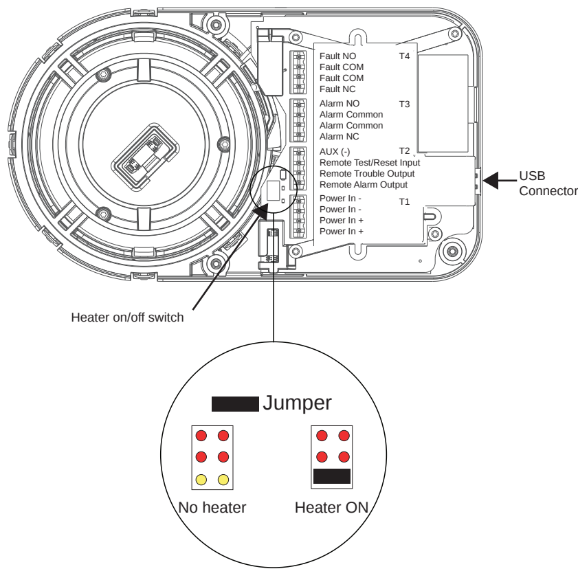
Figure 11-3: Wiring Connections at Detector
