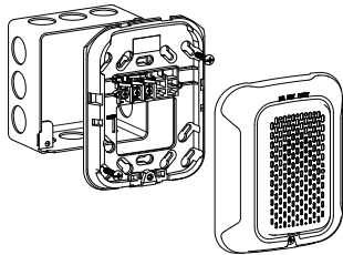
FIGURE 3. STANDARD DEVICE
