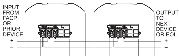
FIGURE 11. 2-WIRE CIRCUIT
