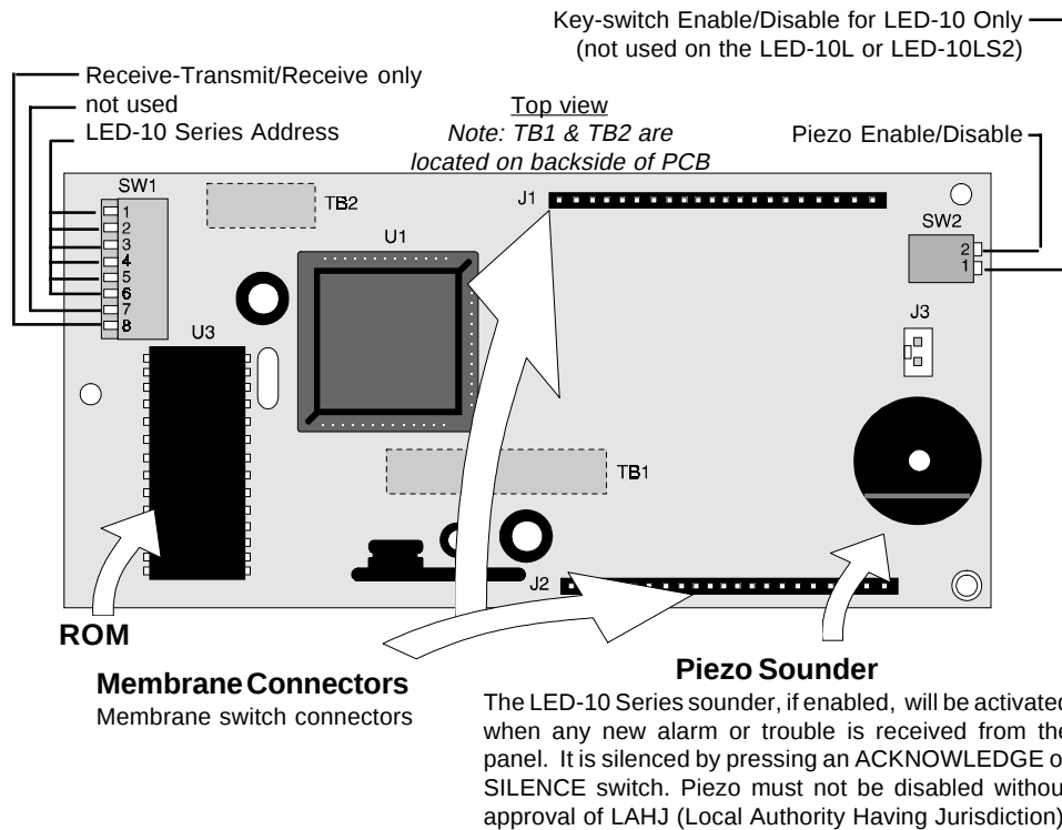
Figure 1-1: Component Summary
