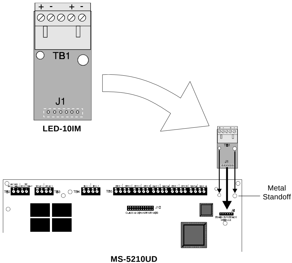
Figure 3-2: LED-10IM Installation
