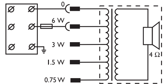
Circuit diagram
