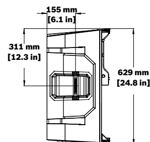
Figure 9.2: ELX200-12P dimensions
