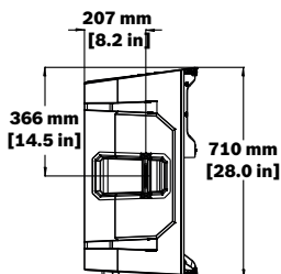
Figure 9.3: ELX200-15P dimensions
