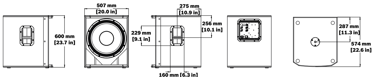
Figure 9.5: ELX200-18SP dimensions
