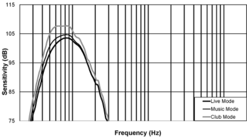
Figure 9.9: ELX200-12SP frequency response: Live, Music, Speech, and Club modes
