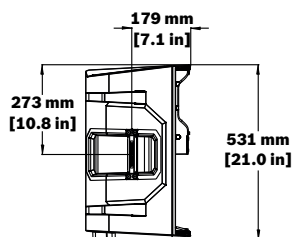
Figure 9.1: ELX200-10P dimensions
