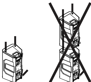
Figure 4.5: Loudspeaker vertical suspension (Correct, left; Incorrect, right)
