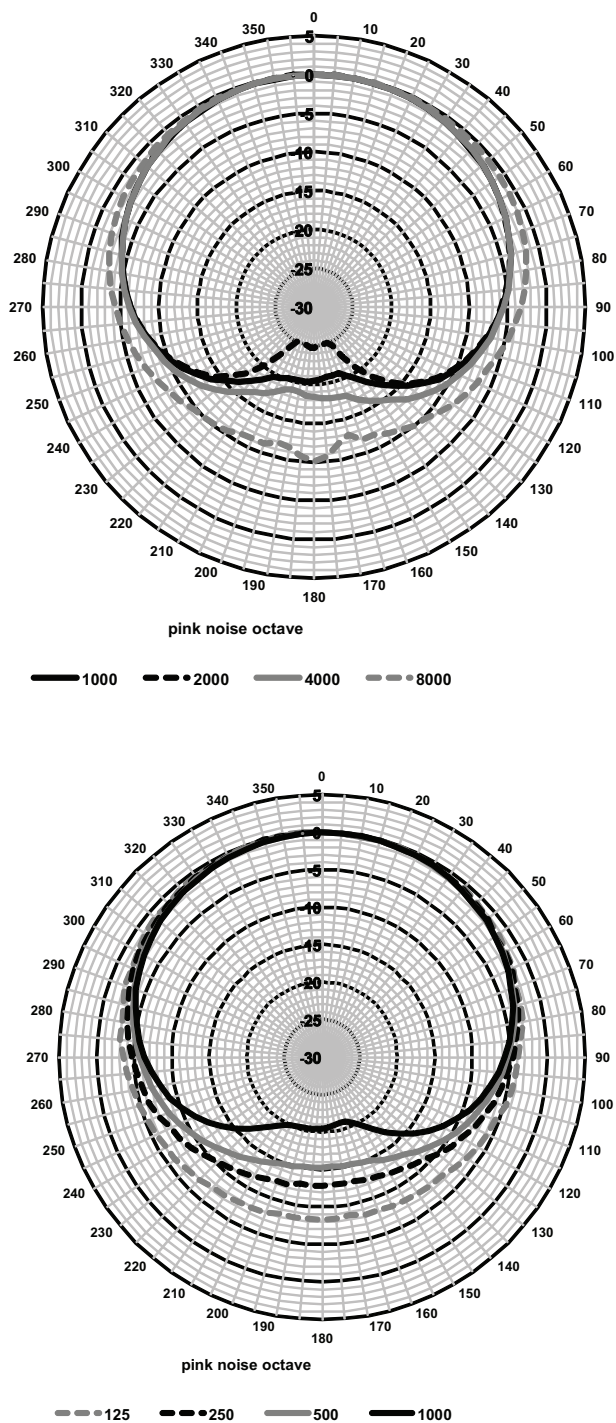
Polar diagram (measured with pink noise)
