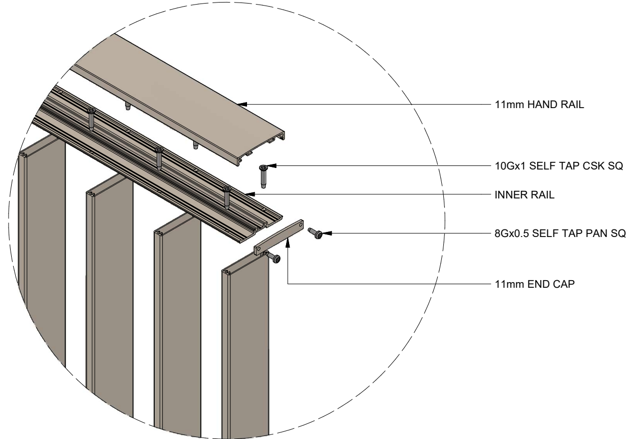
DETAIL D SCALE 1 : 4
