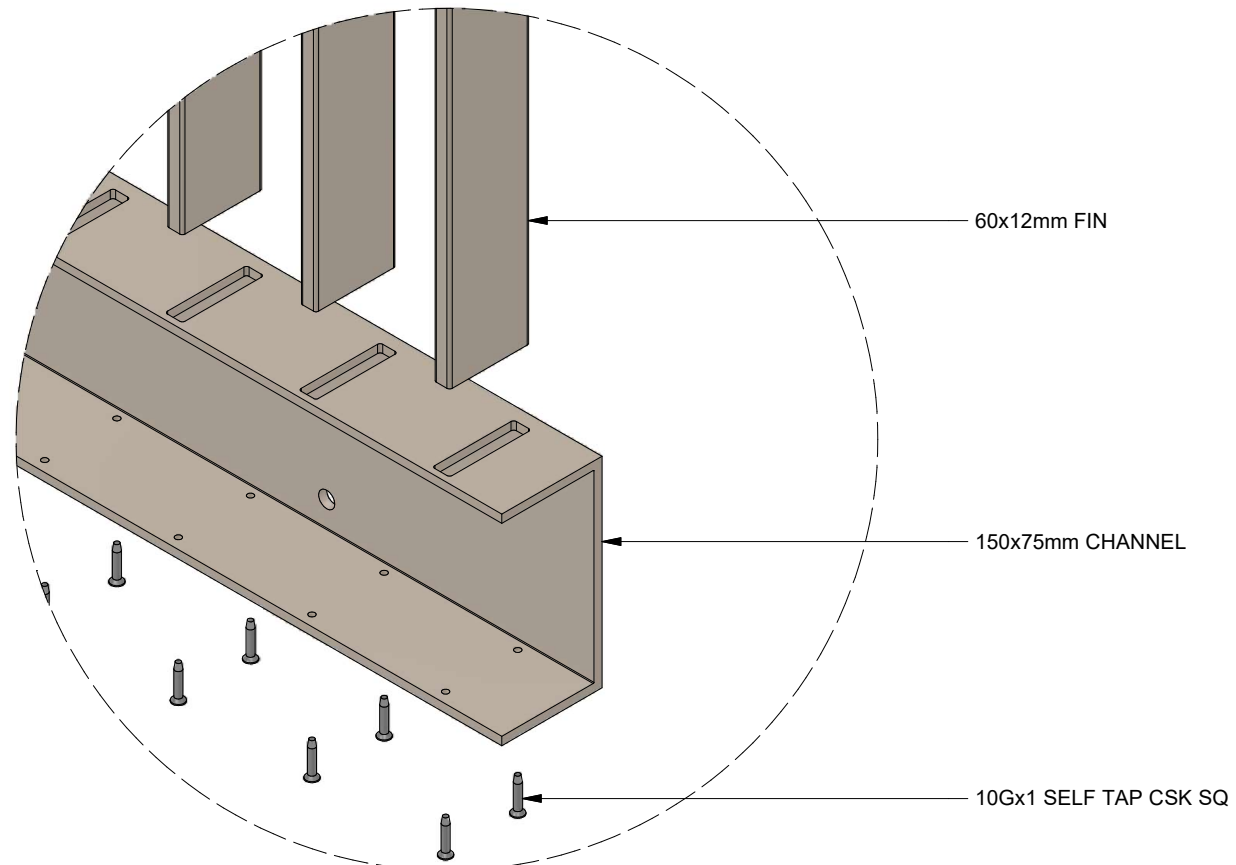
DETAIL E SCALE 1 : 4
