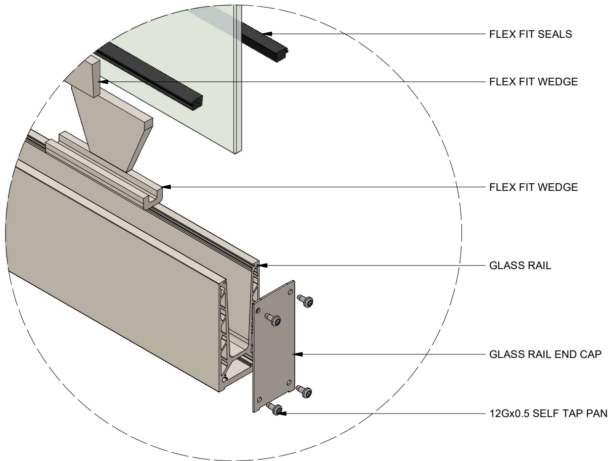
VIEW E
