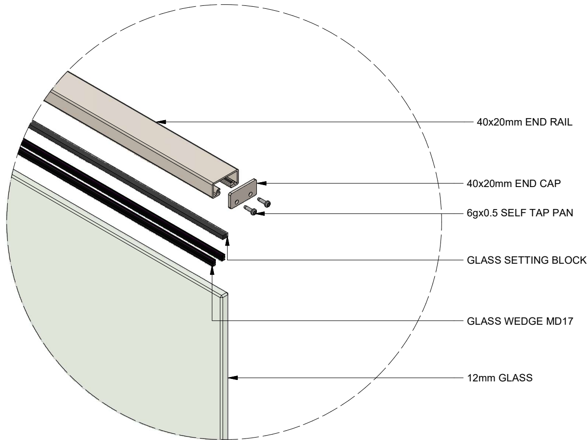
VIEW D
