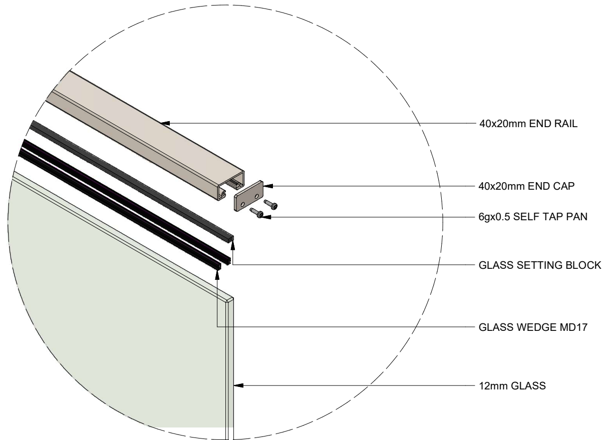
DETAIL D
