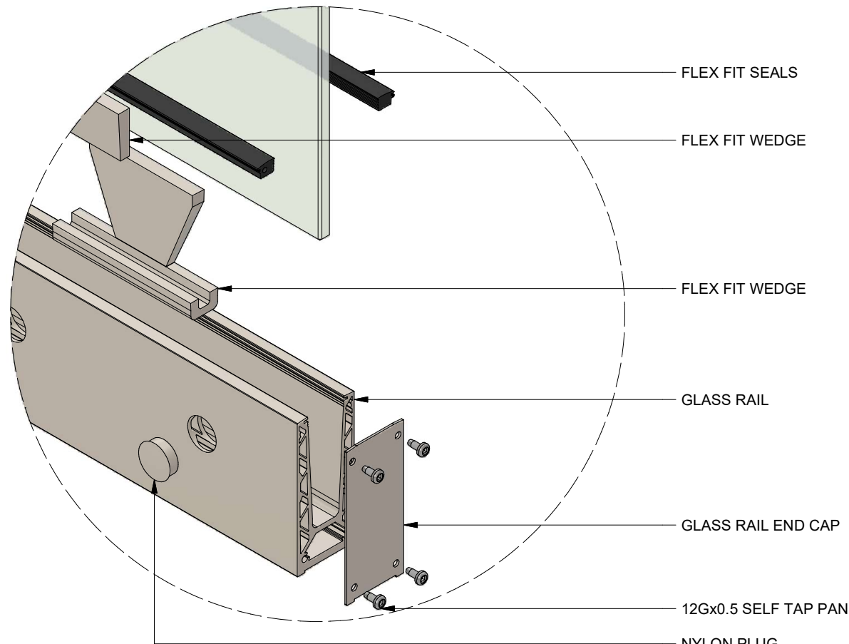
DETAIL E
