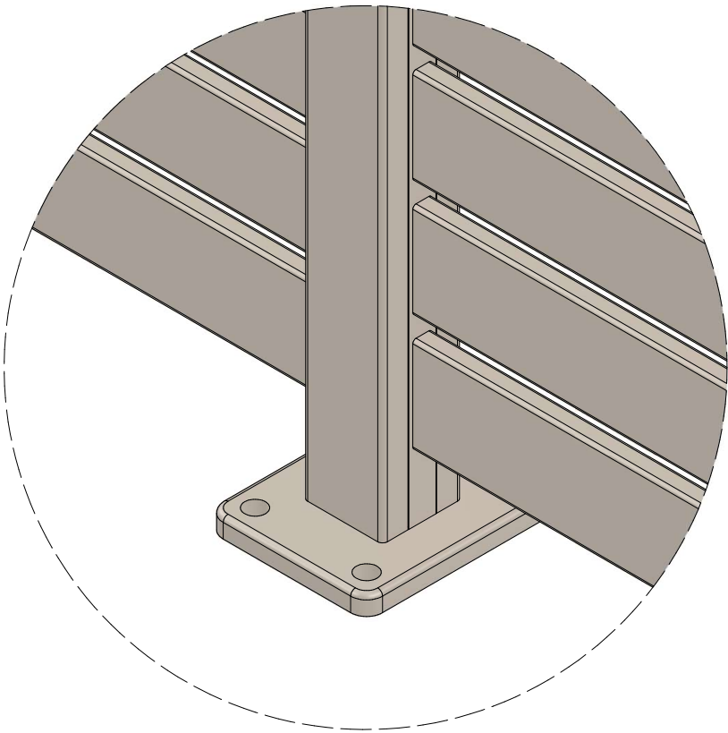
DETAIL C
