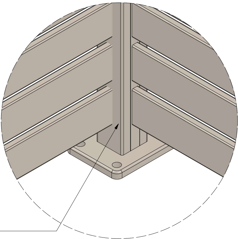
DETAIL B
