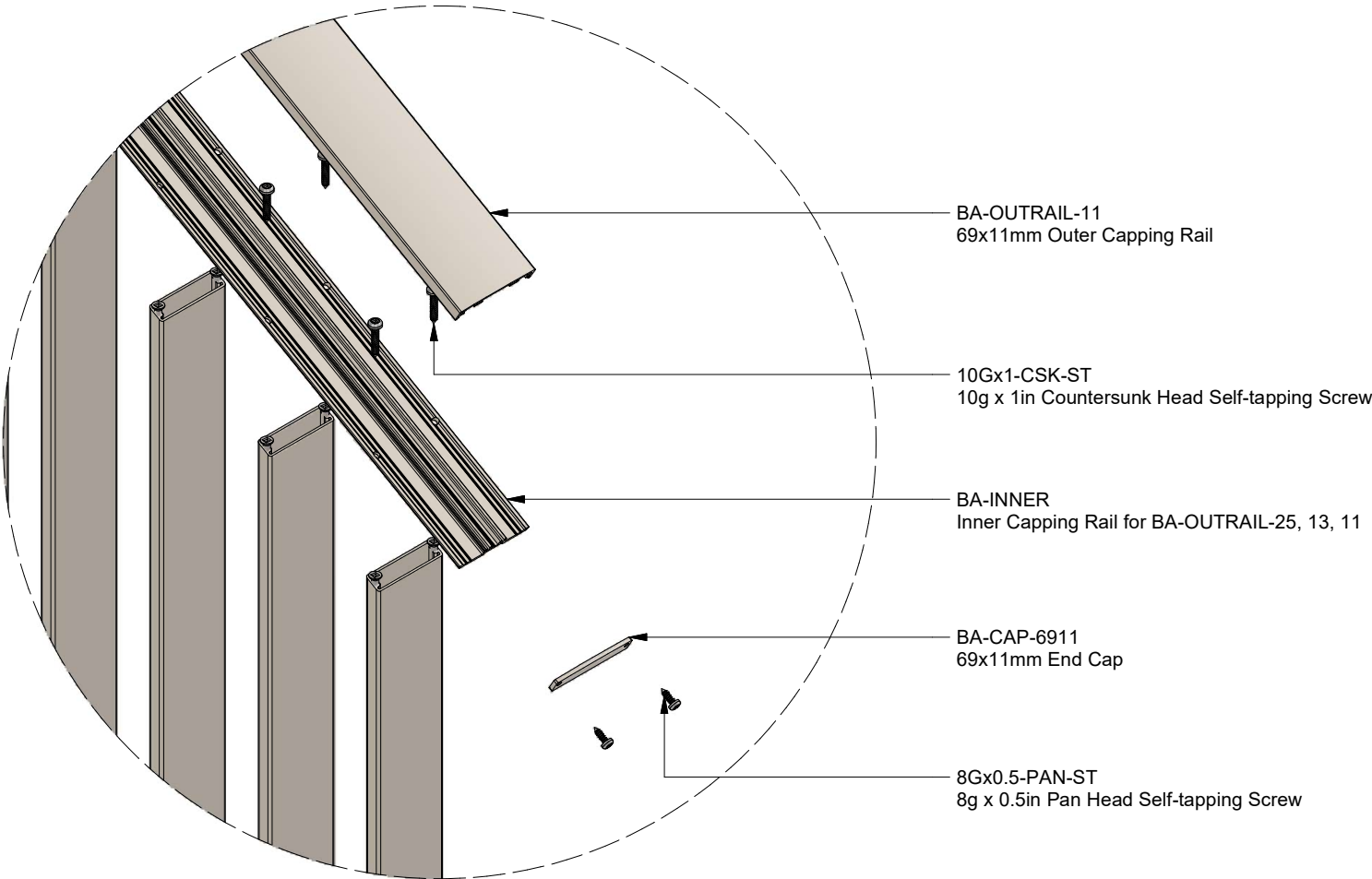
VIEW F
