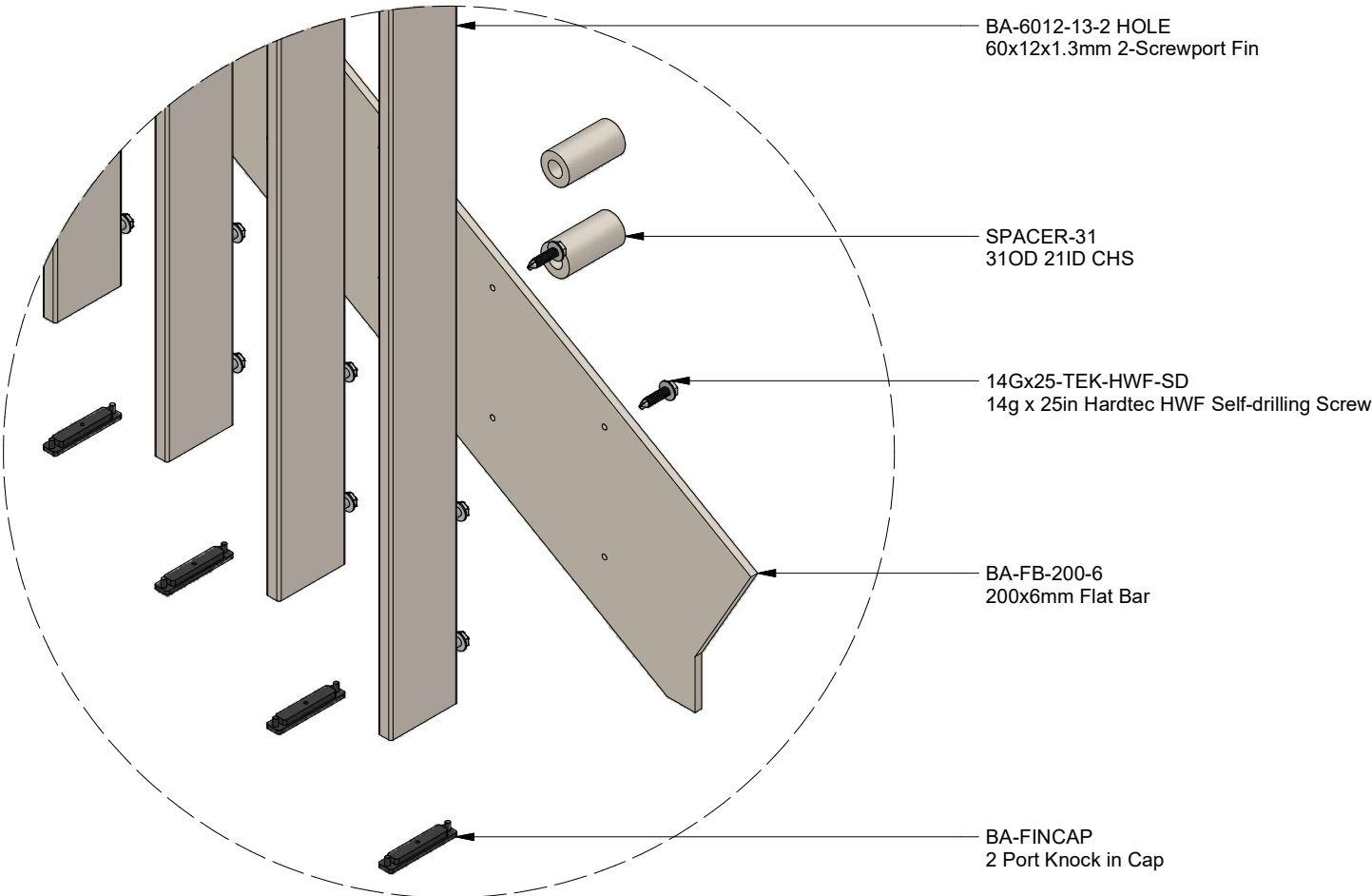
VIEW G
