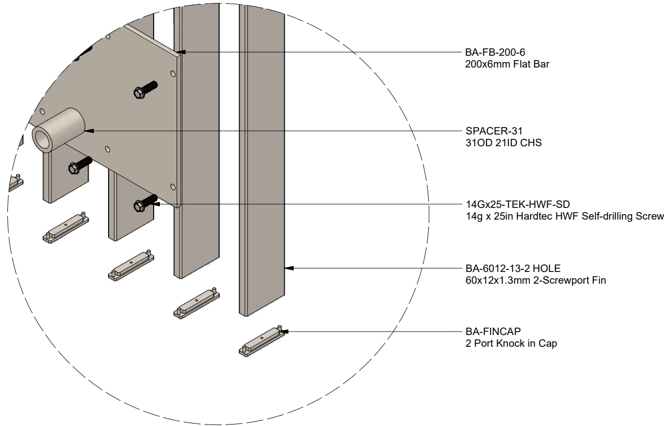
VIEW E
