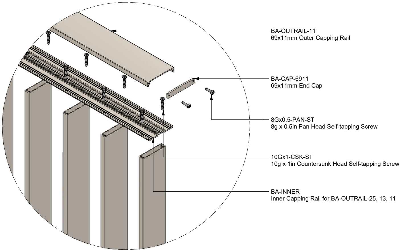
VIEW D
