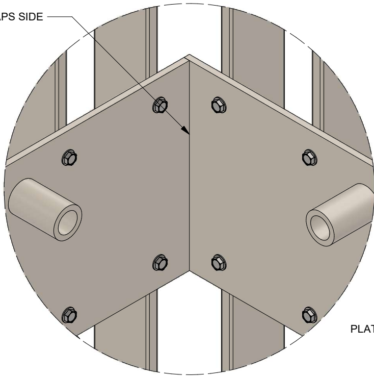
DETAIL B
