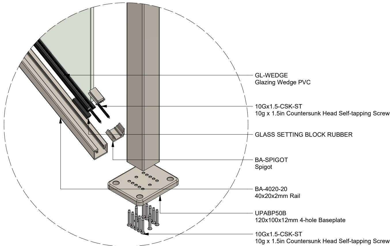
VIEW G
