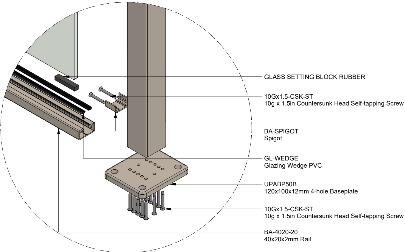
VIEW E
