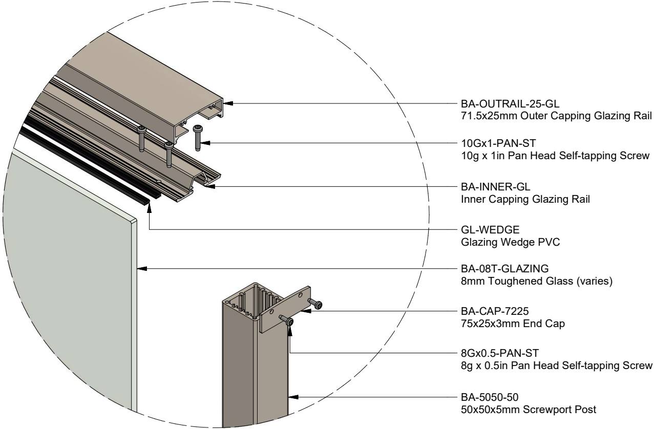
VIEW D
