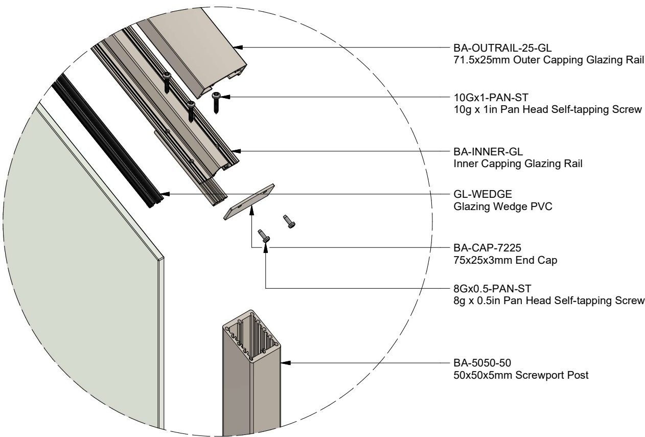
VIEW F
