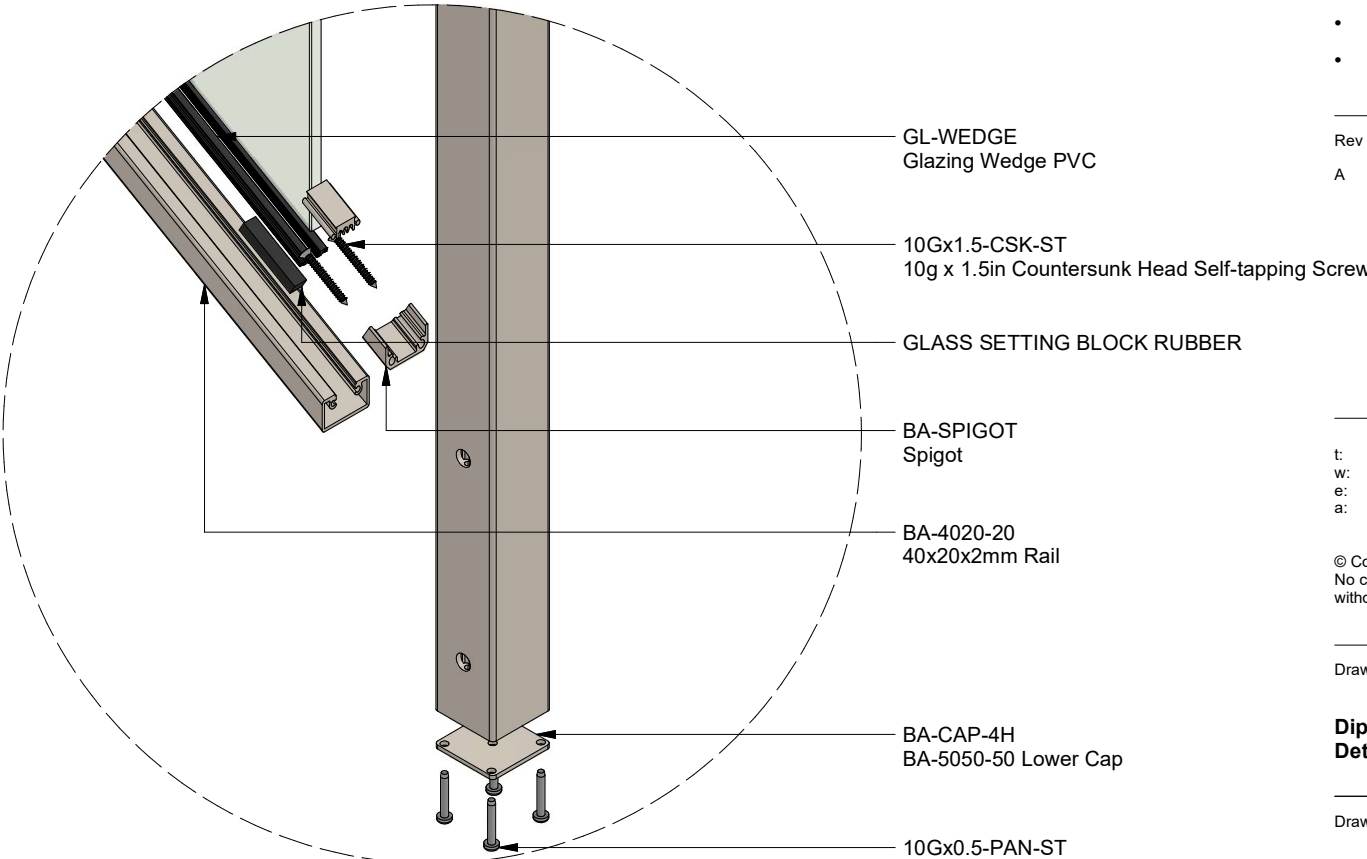
VIEW G
