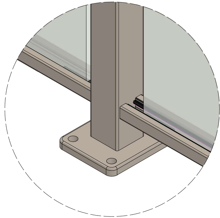
DETAIL C
