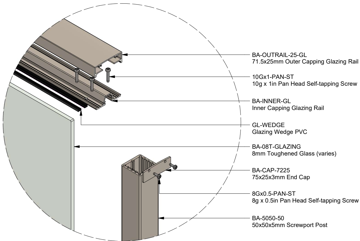
VIEW D
