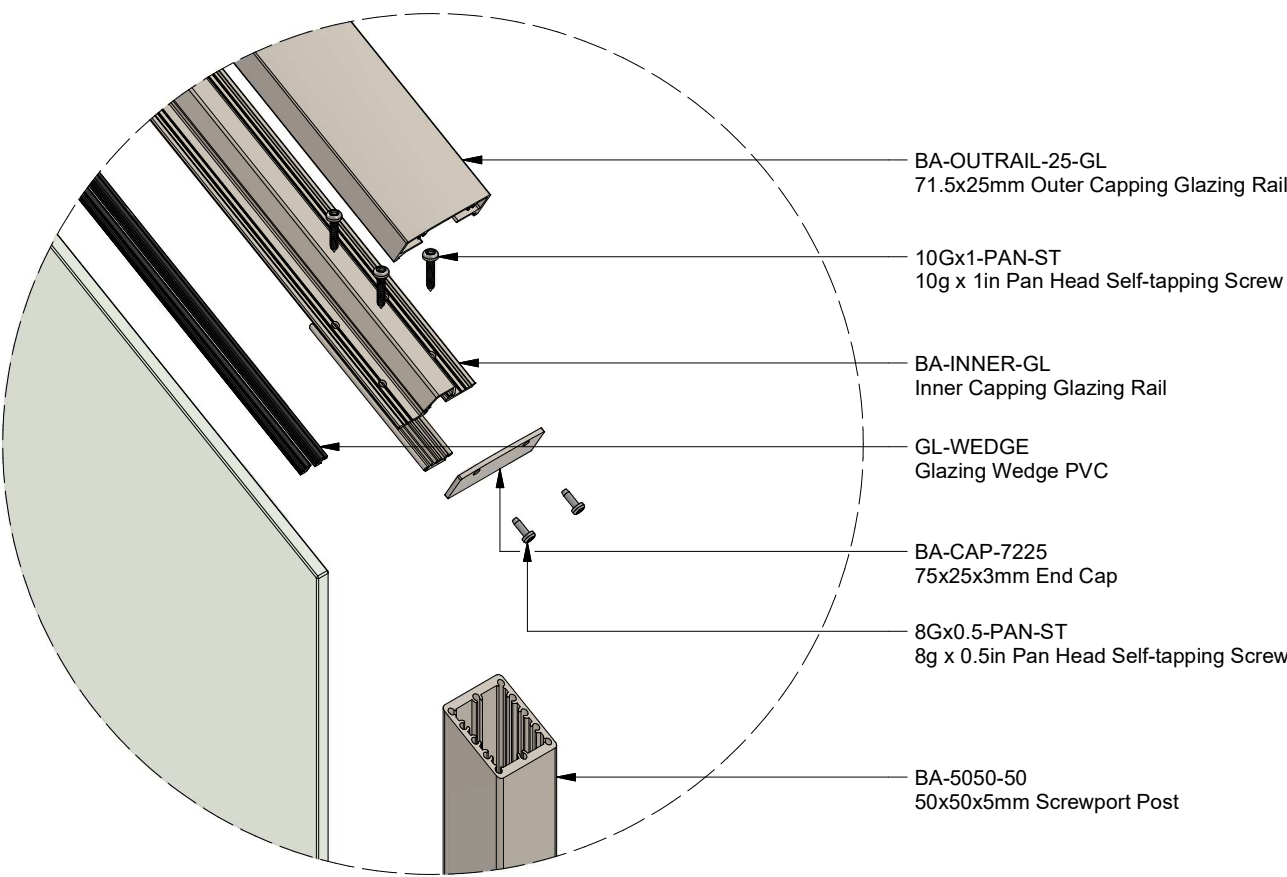
VIEW F
