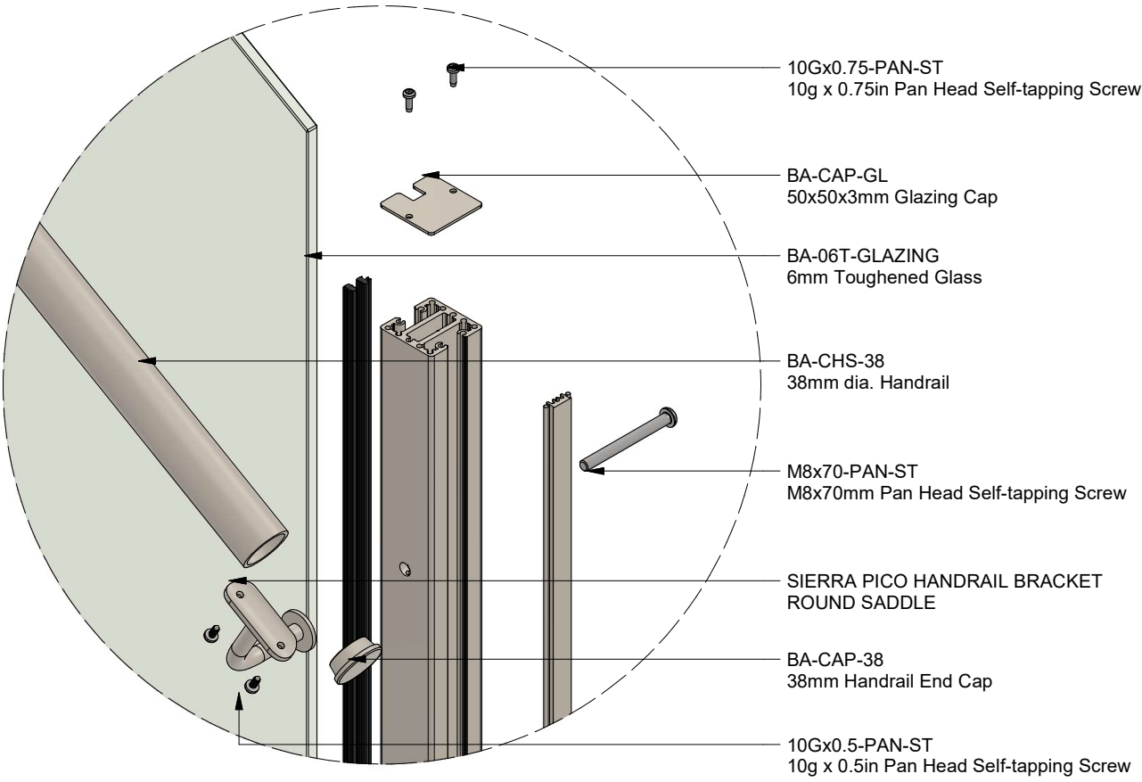
VIEW F
