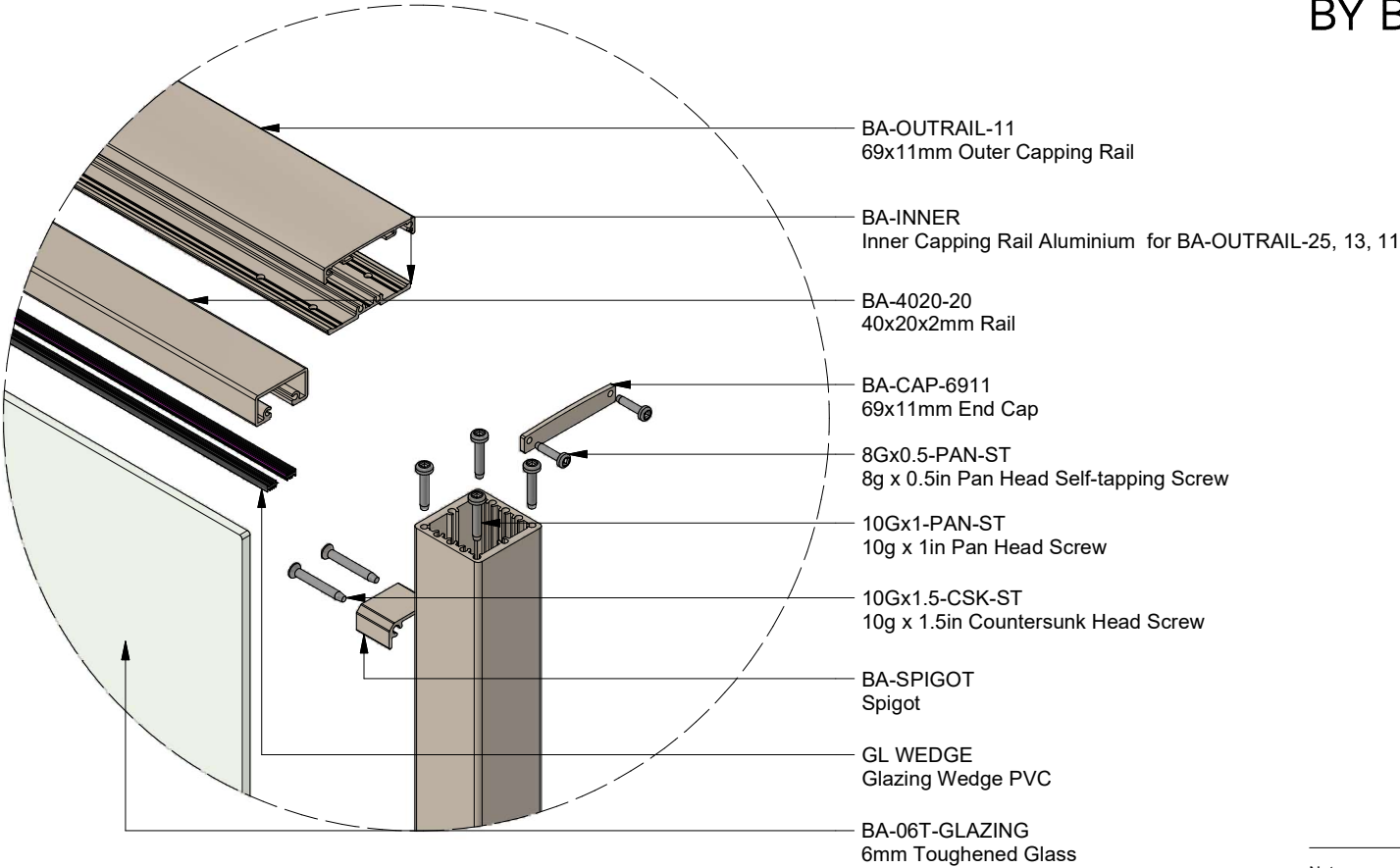
VIEW D
