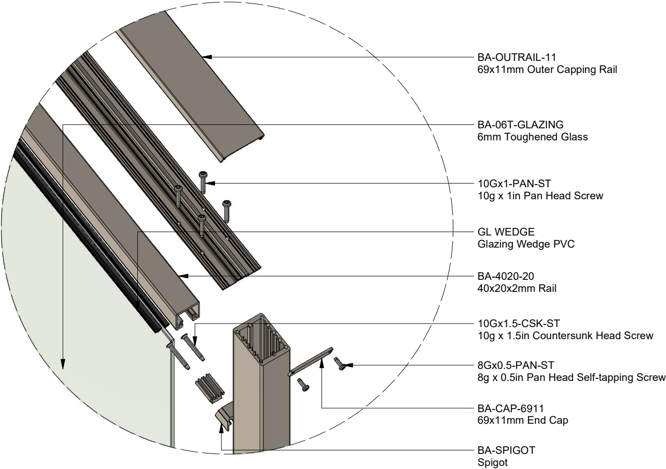
VIEW F
