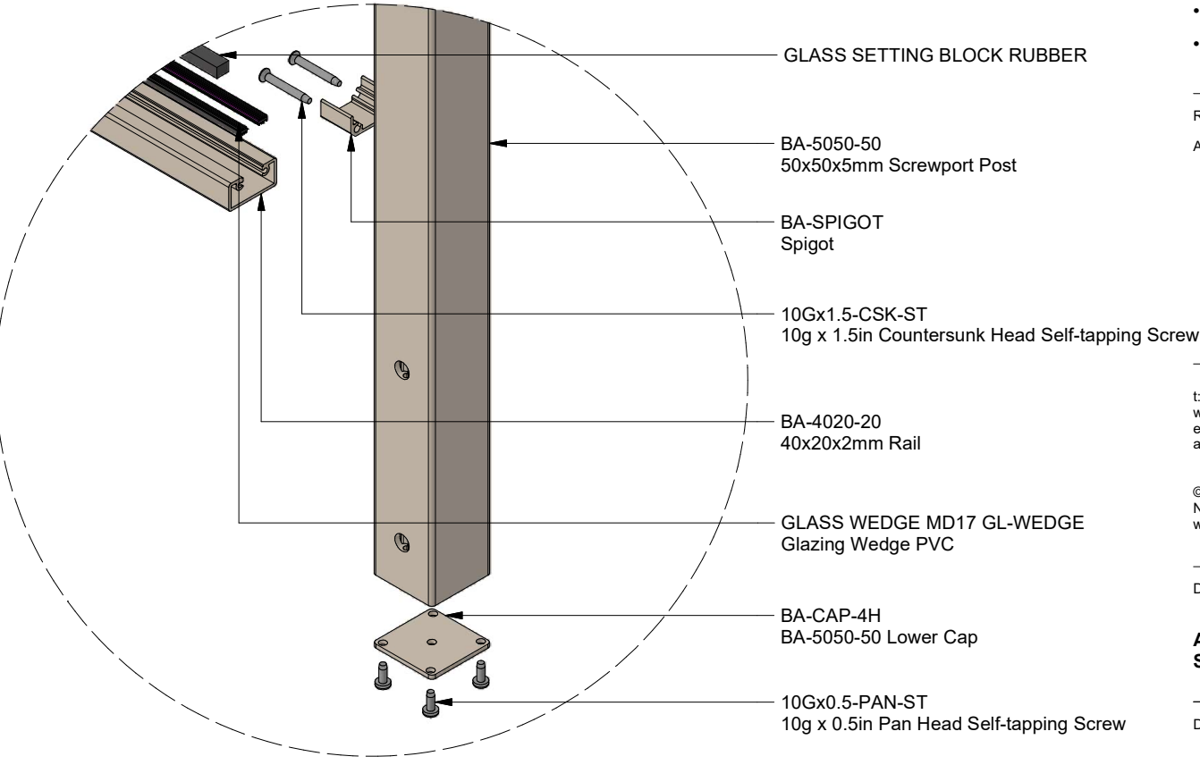
VIEW E
