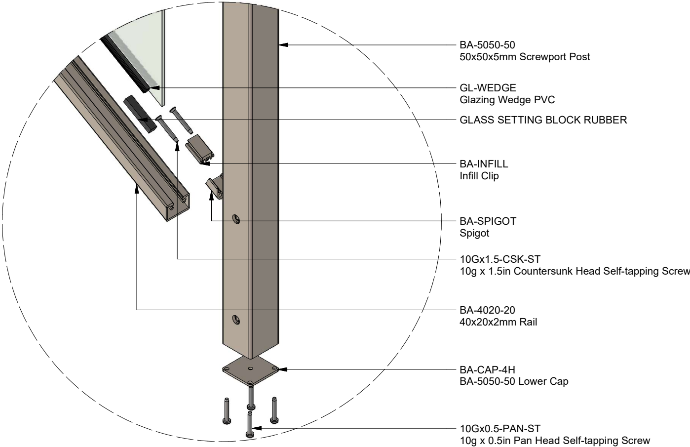
VIEW G
