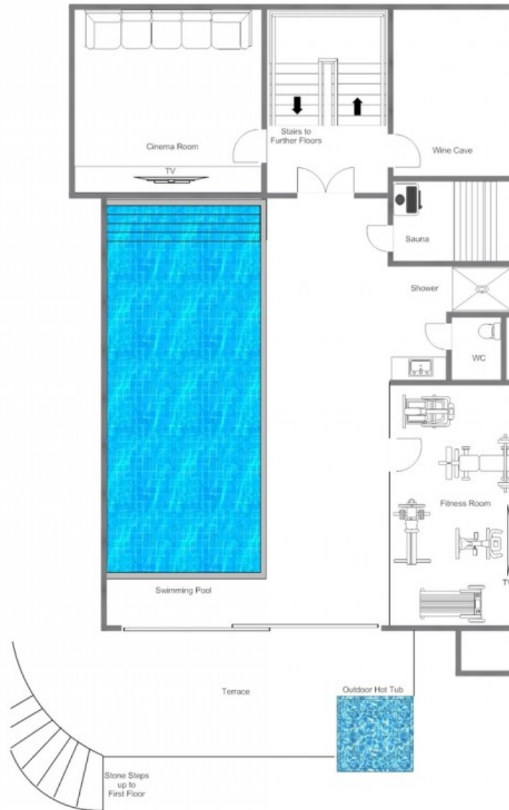
CHALET LA VIGNE - GROUND FLOOR (SPA LEVEL), FOR ILLUSTRATION PURPOSES ONLY
