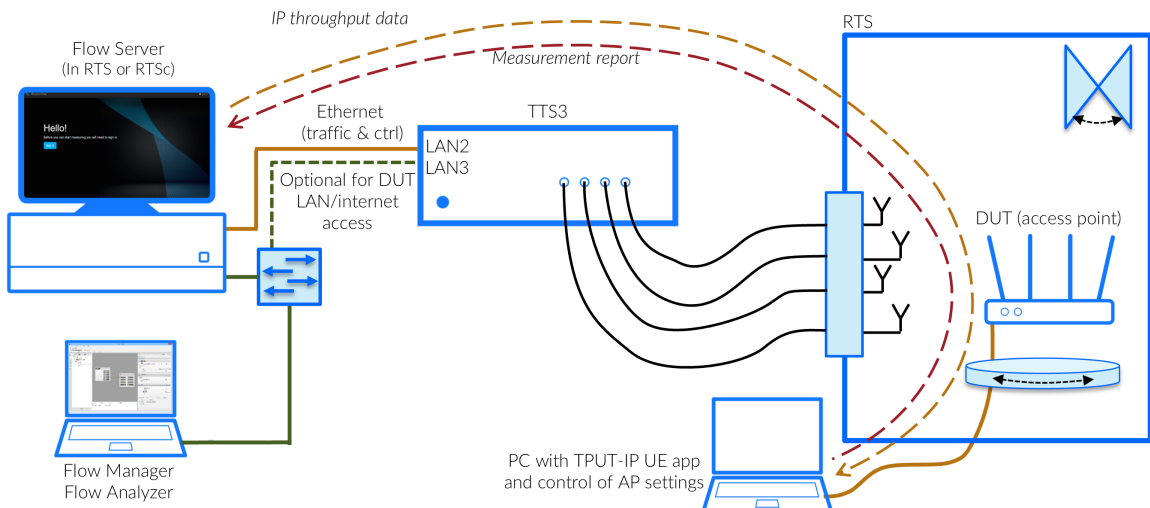
6. System configuration for access point tests with TTS3
