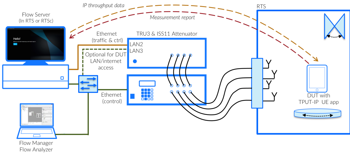
5. System configuration for device tests with TRU3 and ISS11
