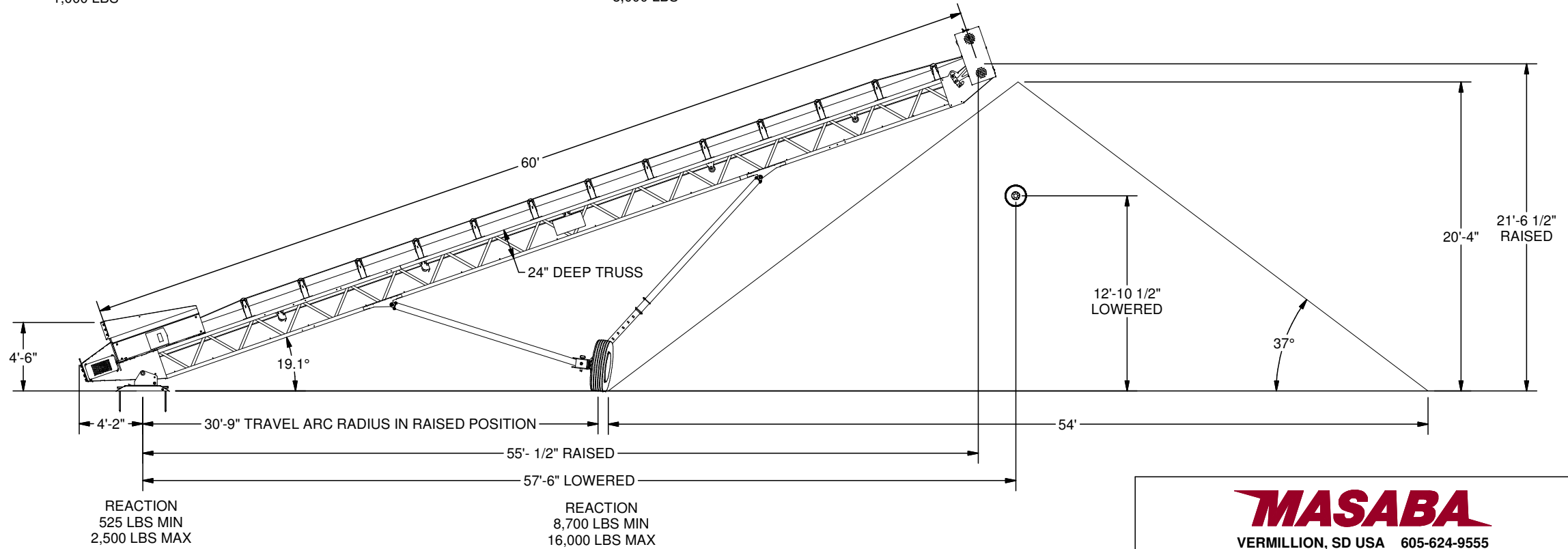
OPERATING POSITION
