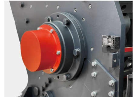
External bearing
