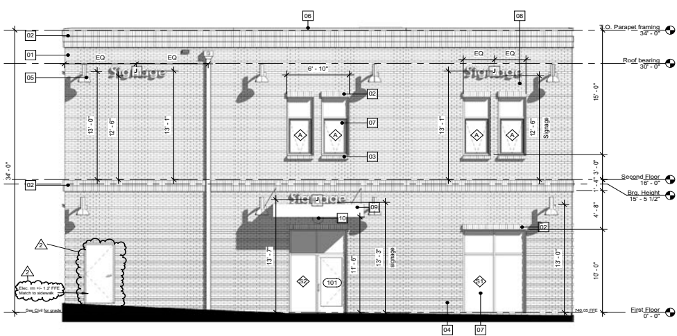
1 ALLEY ELEVATIONS
