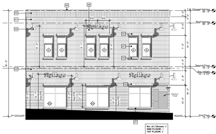
2 EAST ELEVATION (PARKING SIDE)
