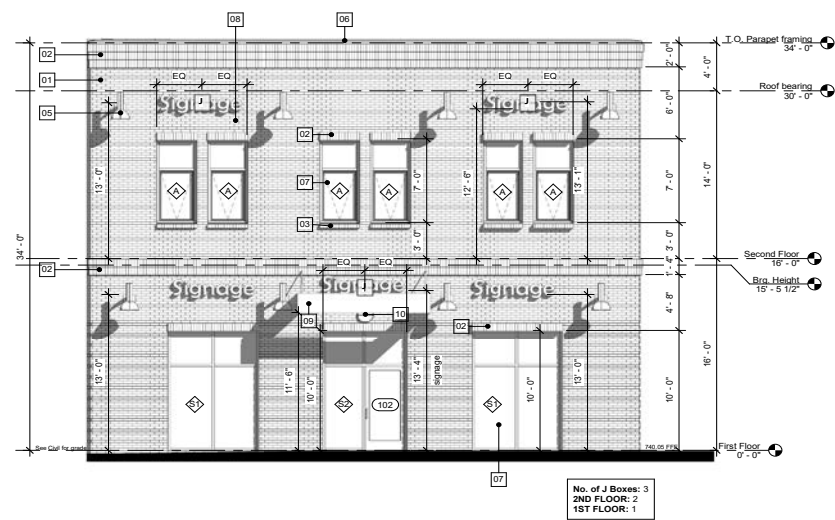
4 STREET ELEVATION
