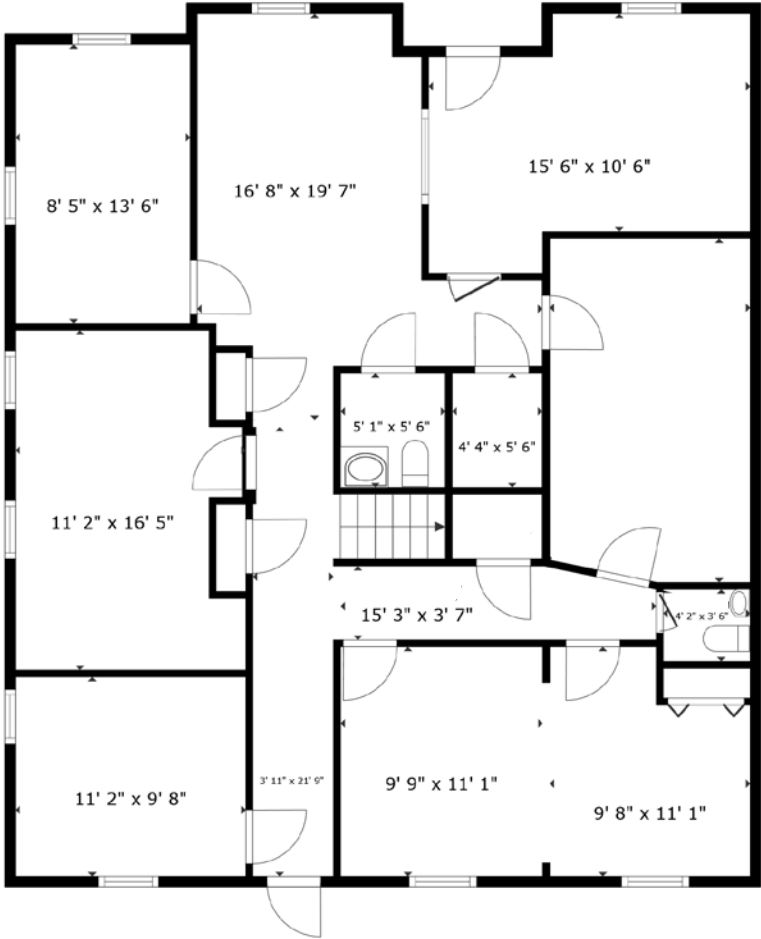
Floor 1
