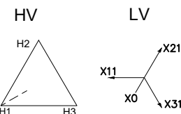
PHASOR DIAGRAM
