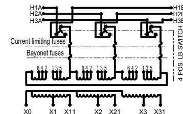
CONNECTION DIAGRAM
