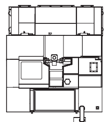
Standard internal rear chip conveyor
