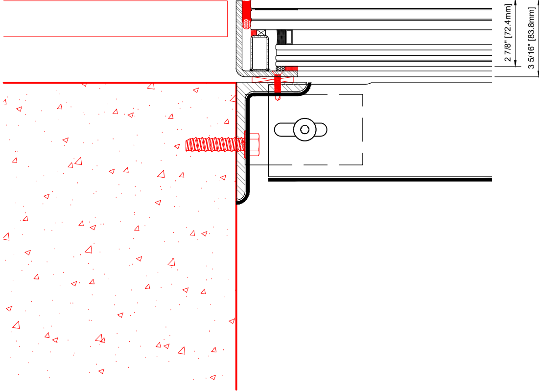
2 1.1 EDGE DETAIL @ CONCRETE SCALE: 3"=1'-0" GREENLITE GLASS INTERIOR DETAILS
