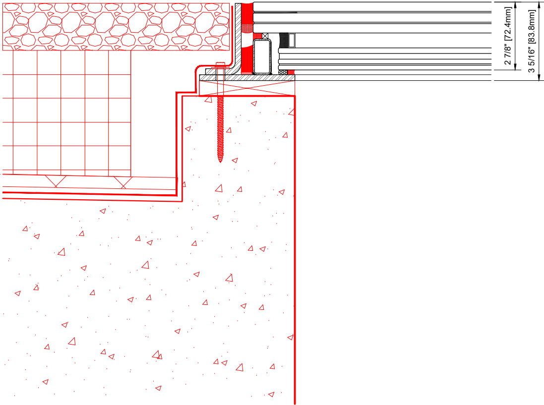
1 1.1 EDGE DETAIL @ CONCRETE SCALE: 3"=1'-0" GREENLITE GLASS EXTERIOR DETAILS
