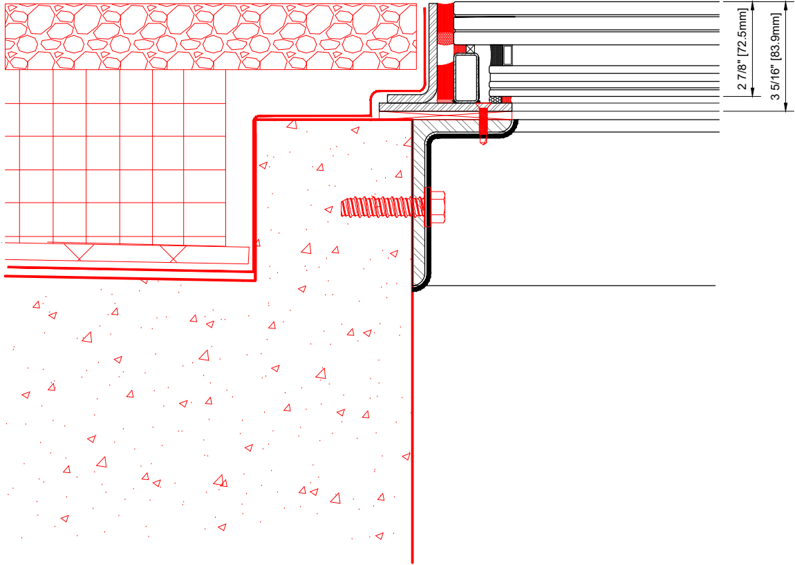
2 1.1 EDGE DETAIL @ CONCRETE SCALE: 3"=1'-0" GREENLITE GLASS EXTERIOR DETAILS
