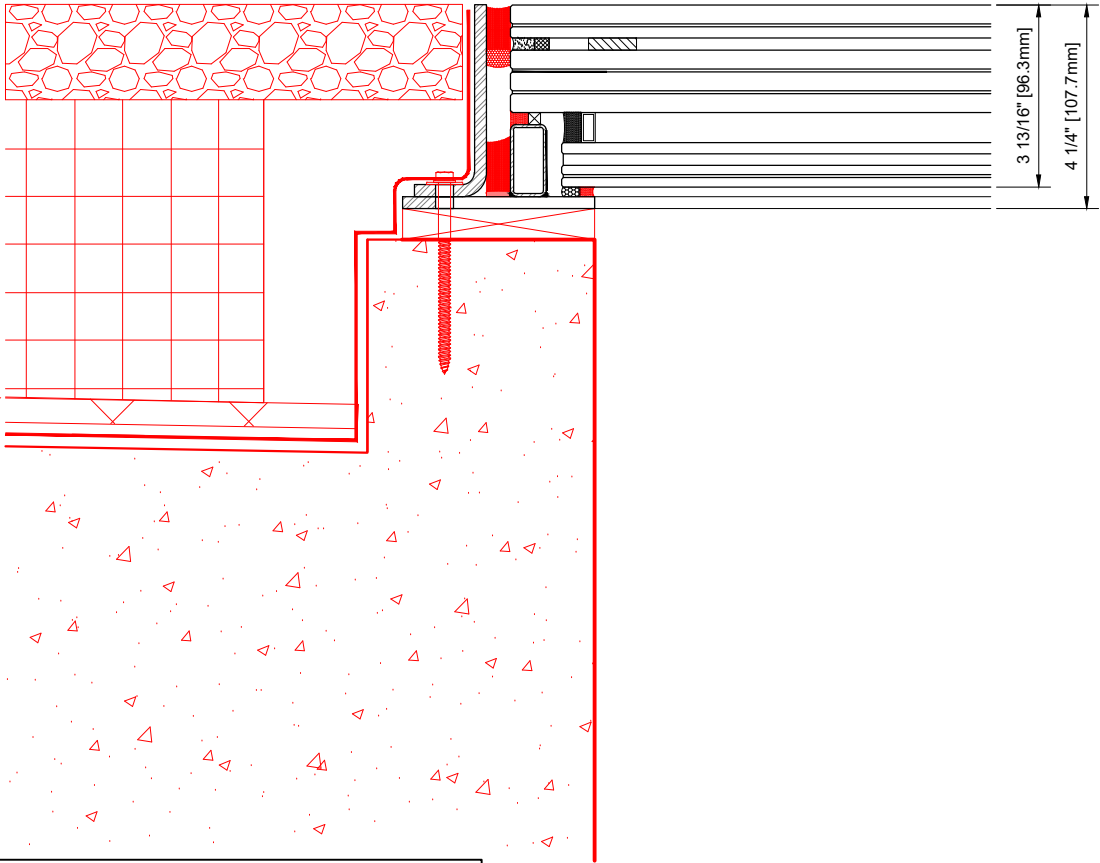
1 1.1 EDGE DETAIL @ CONCRETE SCALE: 3"=1'-0" GREENLITE GLASS EXTERIOR DETAILS
