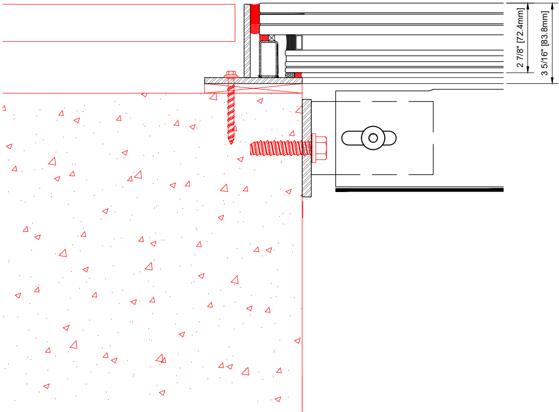
1 1.1 EDGE DETAIL @ CONCRETE SCALE: 3"=1'-0" GREENLITE GLASS INTERIOR DETAILS
