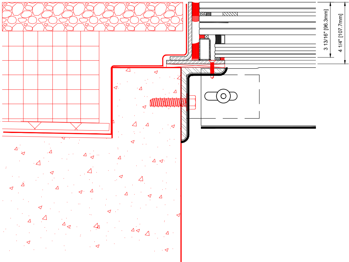
2 1.1 EDGE DETAIL @ CONCRETE SCALE: 3"=1'-0" GREENLITE GLASS EXTERIOR DETAILS
