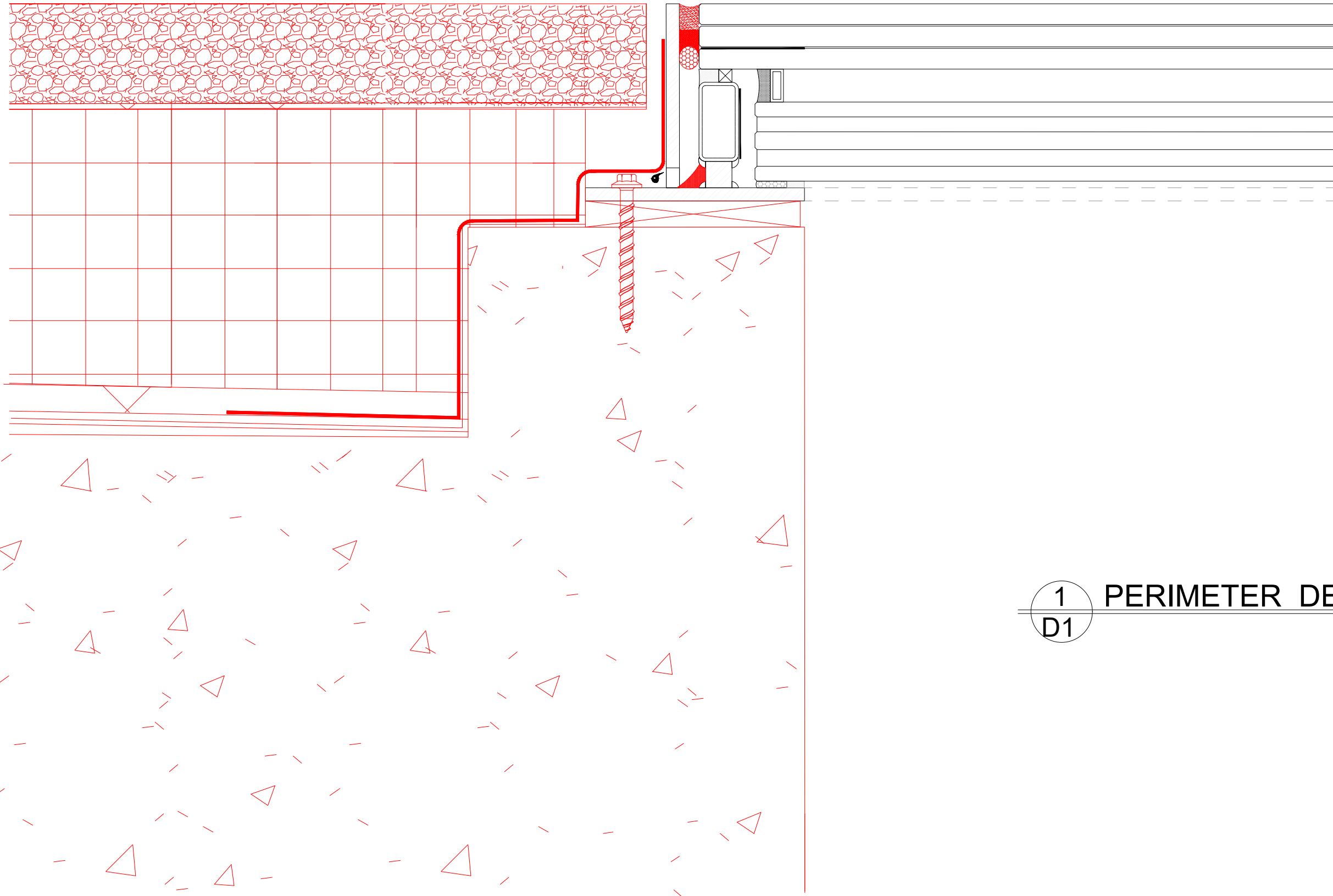
EXTERIOR DETAIL
