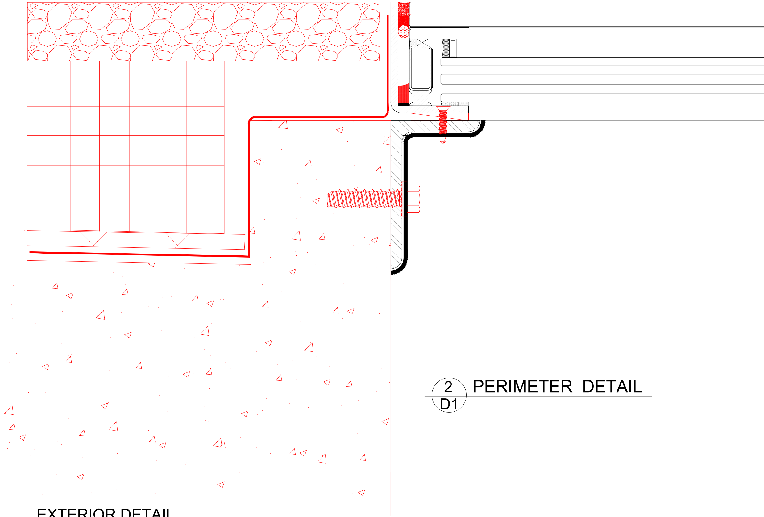
EXTERIOR DETAIL
