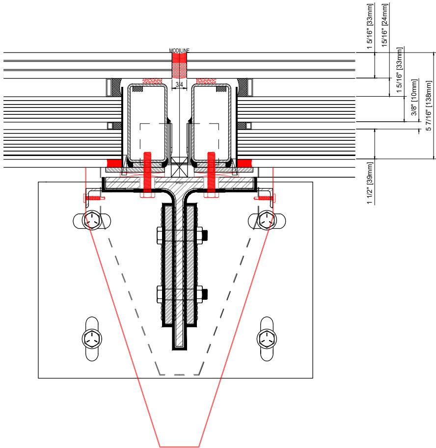
3 SECONDARY BEAM CONNECTION SCALE: 2-1/2"=1'-0" GREENLITE GLASS EXTERIOR DETAILS
