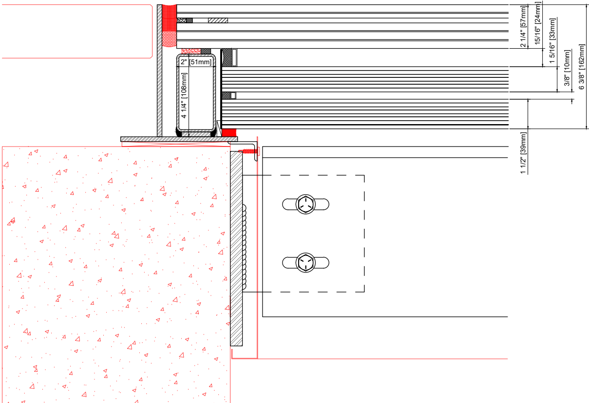
1 1.1 EDGE DETAIL @ CONCRETE SCALE: 2-1/2"=1'-0" GREENLITE GLASS INTERIOR DETAILS
