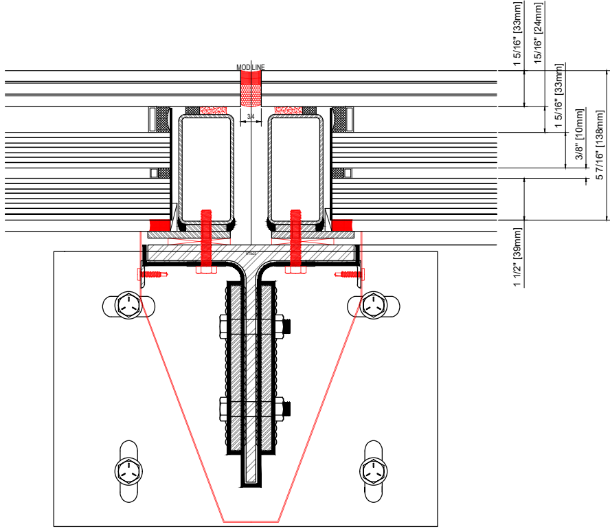
1 1.1 EDGE DETAIL @ CONCRETE SCALE: 2-1/2"=1'-0" GREENLITE GLASS INTERIOR DETAILS
