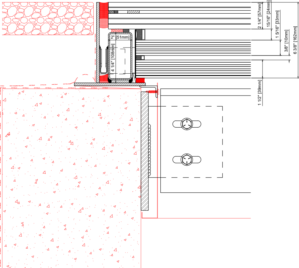
1 1.1 EDGE DETAIL @ CONCRETE SCALE: 2-1/2"=1'-0" GREENLITE GLASS EXTERIOR DETAILS
