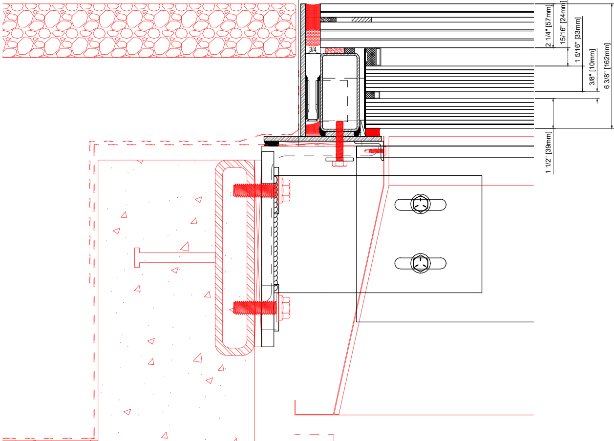
2 1.1 EDGE DETAIL @ CONCRETE SCALE: 2-1/2"=1'-0" GREENLITE GLASS EXTERIOR DETAILS
