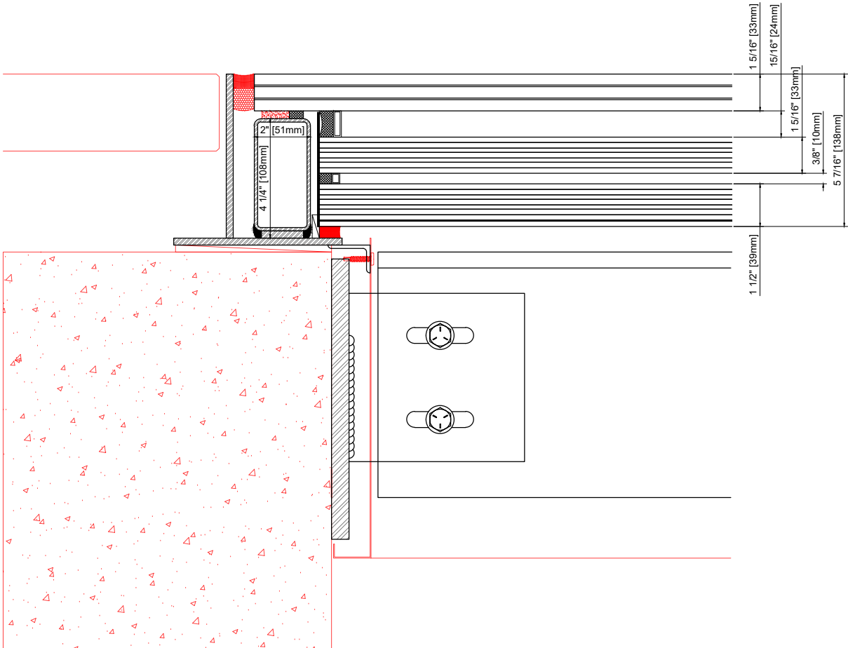
1 1.1 EDGE DETAIL @ CONCRETE SCALE: 2-1/2"=1'-0" GREENLITE GLASS INTERIOR DETAILS
