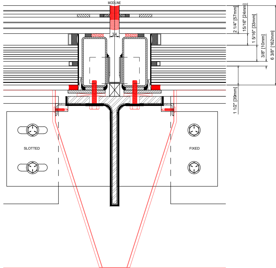
4 1.1 PRIMARY BEAM CONNNECTION SCALE: 2-1/2"=1'-0" GREENLITE GLASS EXTERIOR DETAILS
