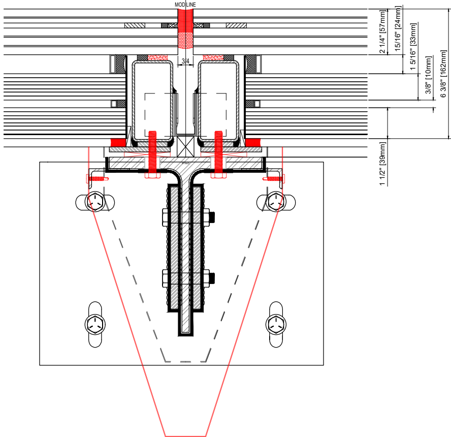
3 1.1 SECONDARY BEAM CONNECTION SCALE: 2-1/2"=1'-0" GREENLITE GLASS EXTERIOR DETAILS
