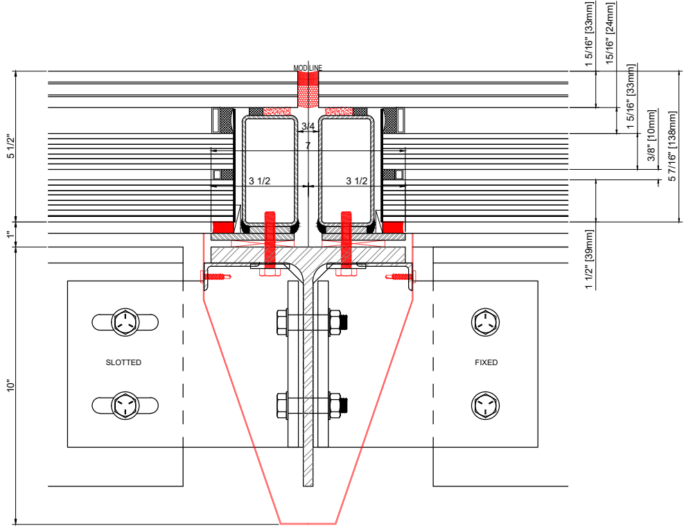
2 1.1 EDGE DETAIL @ CONCRETE SCALE: 2-1/2"=1'-0" GREENLITE GLASS EXTERIOR DETAILS
