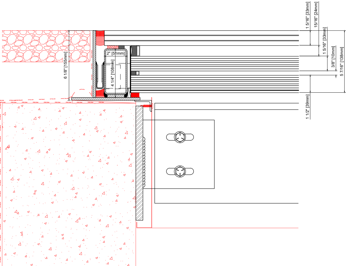
1 EDGE DETAIL @ CONCRETE SCALE: 2-1/2"=1'-0" GREENLITE GLASS EXTERIOR DETAILS
