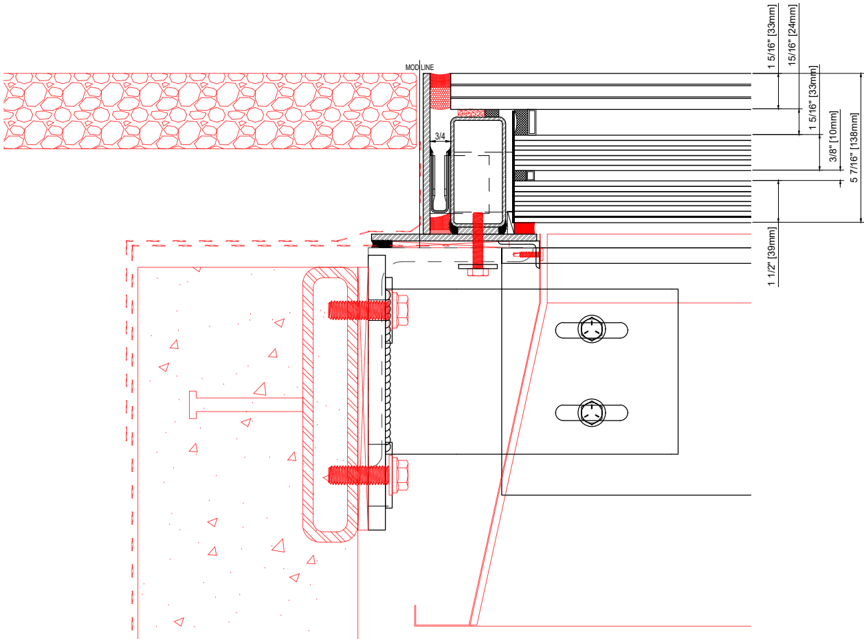
2 EDGE DETAIL @ CONCRETE SCALE: 2-1/2"=1'-0" GREENLITE GLASS EXTERIOR DETAILS
