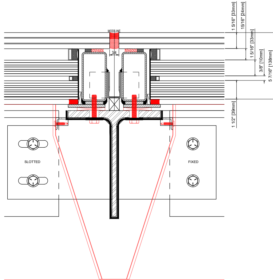
4 PRIMARY BEAM CONNECTION SCALE: 2-1/2"=1'-0" GREENLITE GLASS EXTERIOR DETAILS
