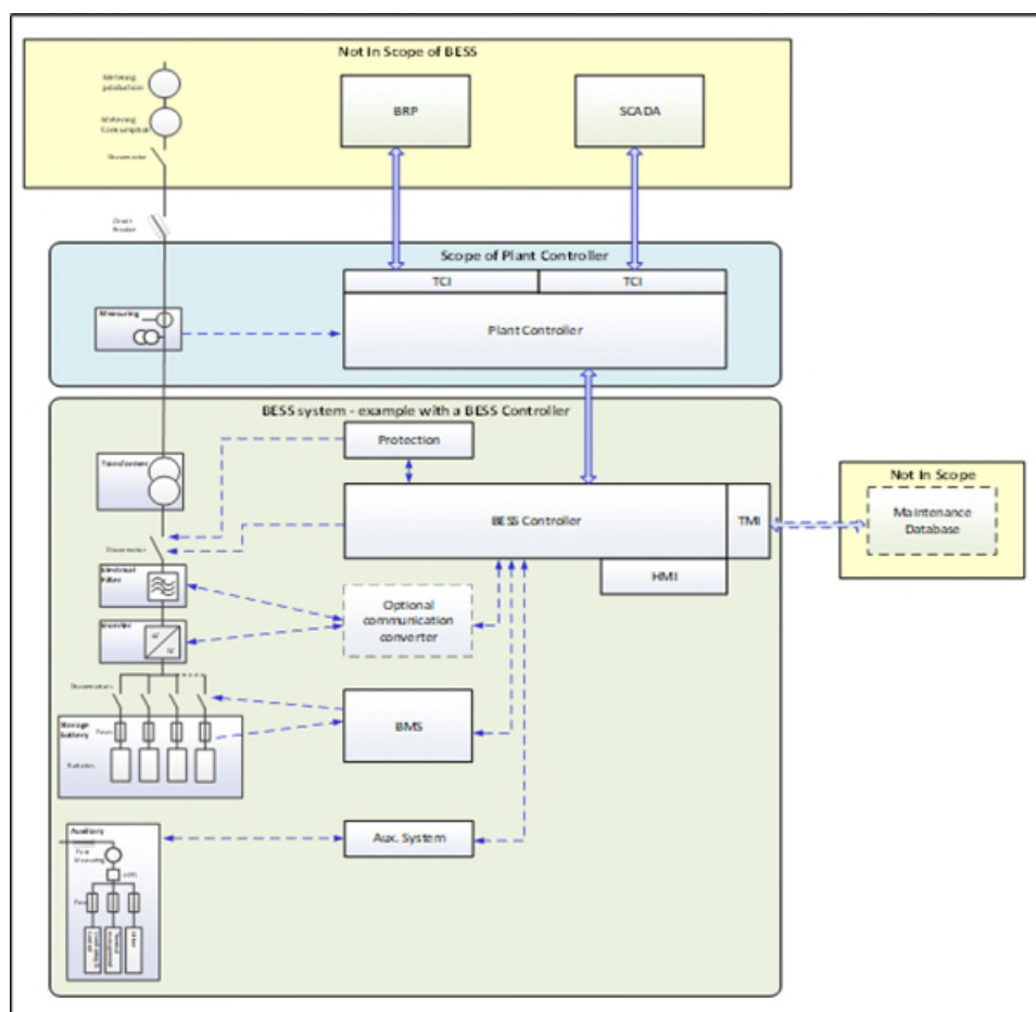
FIGURE 15: SYSTEM BOUNDARIES FOR BESS AND GRID INTEGRATION (SOURCE: K. NØRREGAARD, DTI)
