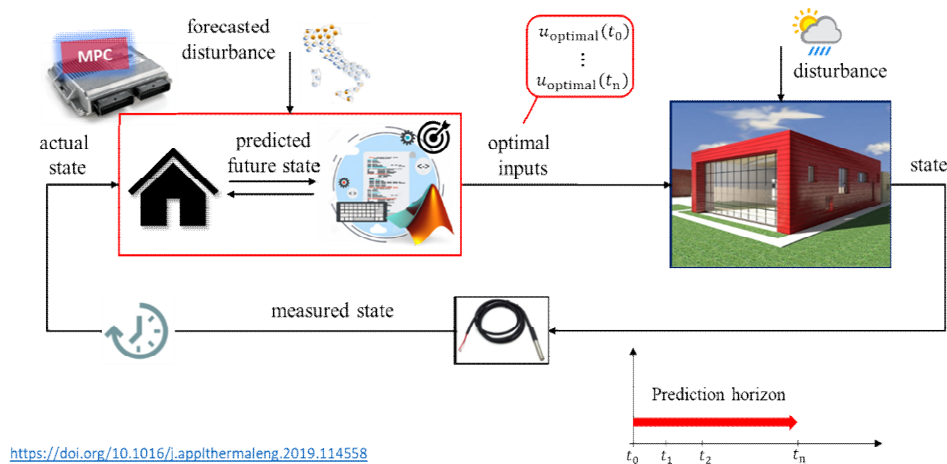
FIGURE 10: CONCEPT OF A MODEL PREDICTIVE CONTROL (SOURCE: M. MORINI, UNIPR)
