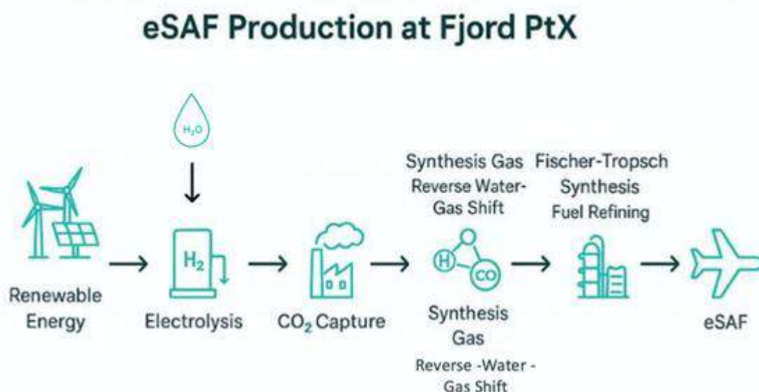
Figure 41 eSAF Production at Fjord PtX 62
