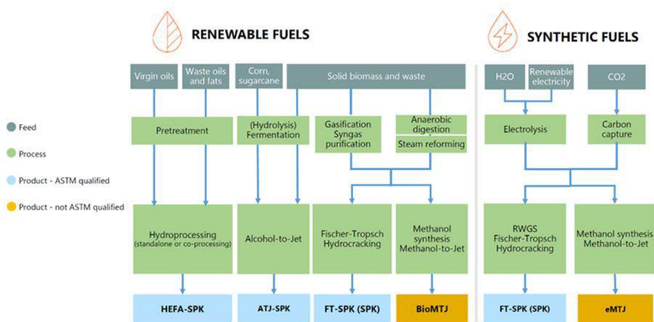
Figure 39 Main SAF production pathways with similar building blocks 147
