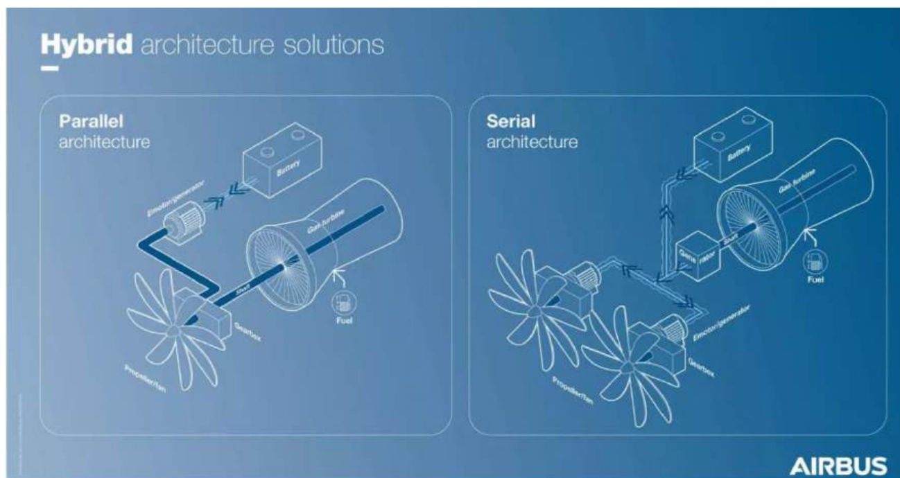
Figure 55 Hybrid architecture solutions, Airbus 189 (Other models and combinations can be found on ResearchGate ) 190
