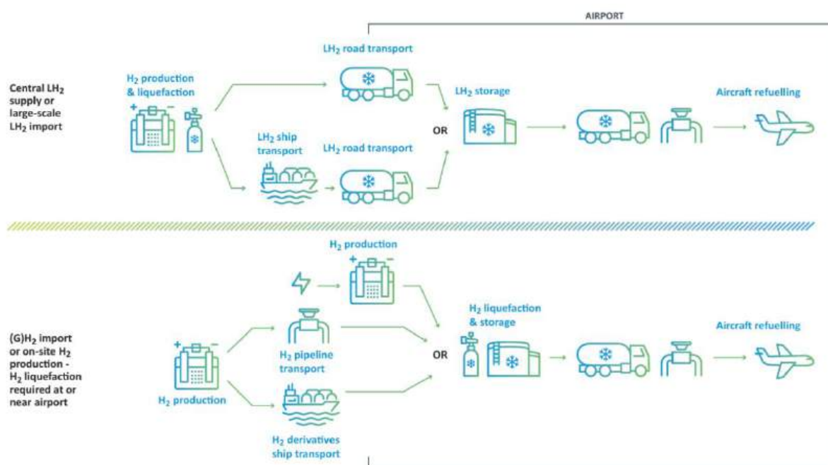
Figure 56 Energy supply models for hydrogen to the airfield 191
