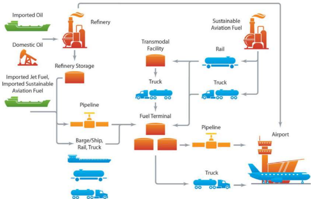
Figure 2 Illustration of SAF distribution 3
