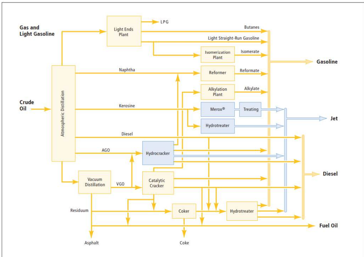
Figure 1 Schematic of a modern conventional oil refinery 1
