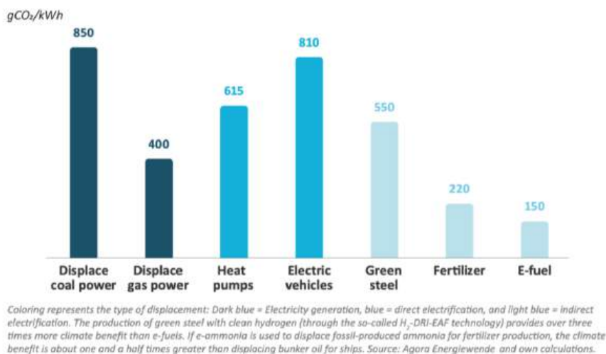
Figure 50 Climate impact of using clean electricity to displace fossil energy for various purposes 177
