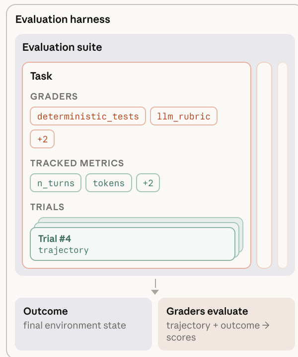
Components of evaluations for agents.
