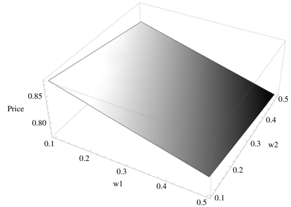
(b) Analysis II: price of the bond (Z axis) as the function of w_1 (X axis) and w_2 (Y axis).
