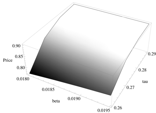
(a) Analysis I: price of the bond (Z axis) as the function of \beta_W (X axis) and \tau_W (Y axis).
