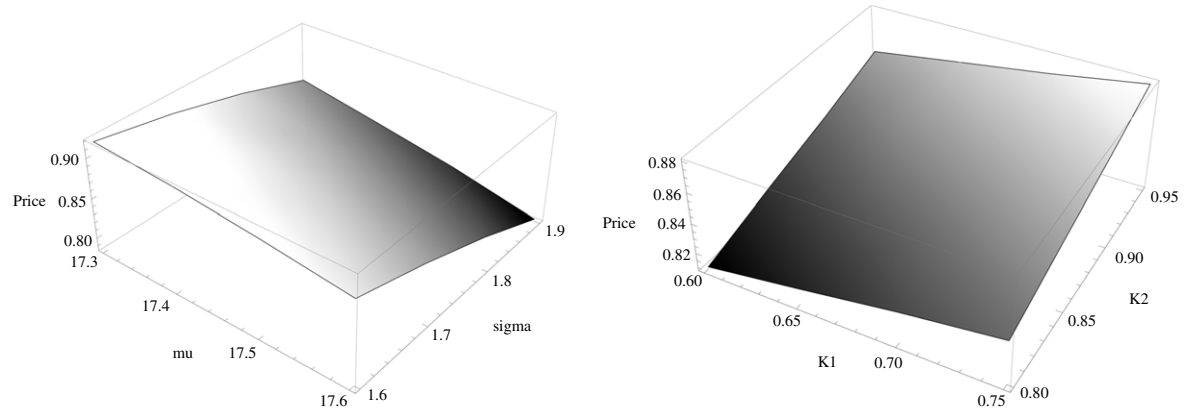
(a) Analysis I: price of the bond (Z axis) as the function of \mu_{LN} (X axis) and \sigma_{LN} (Y axis).
