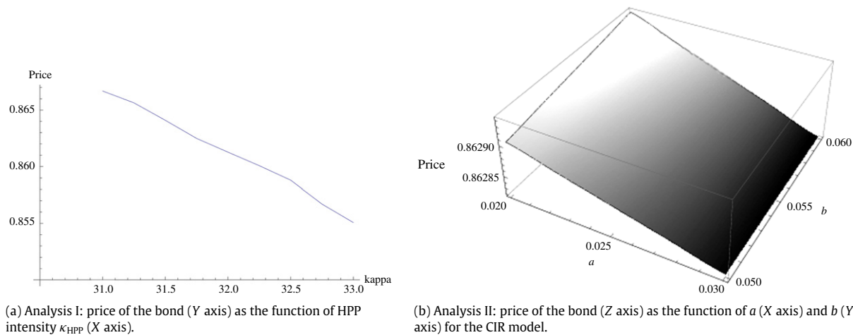
Fig. 4. Graphs for numerical analysis of Model IV.
