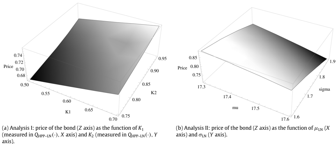
Fig. 3. Graphs for numerical analysis of Model III.
