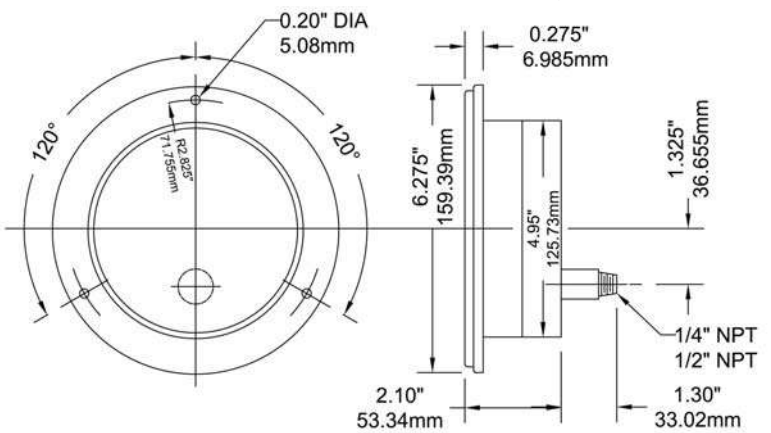
4.5" Back Connection with Standard Front Flange
