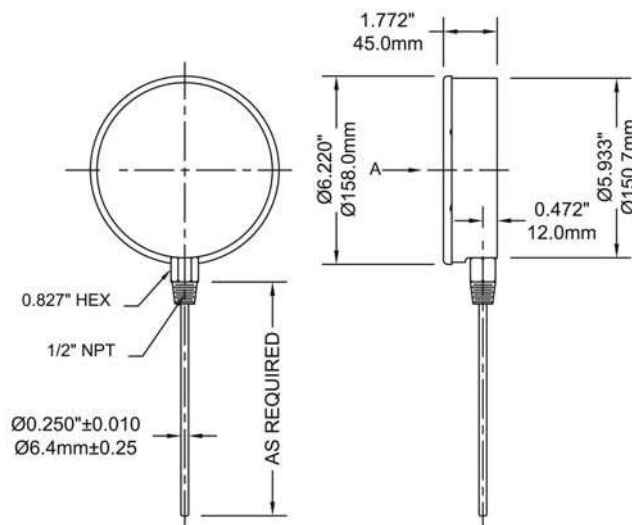
6" Bottom Connection
