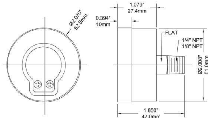
2" Back Connection
