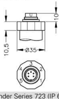
Binder Series 723 (IP 67)
