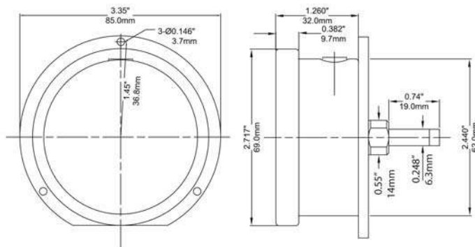
2.5" Back Connection with Back Flange
