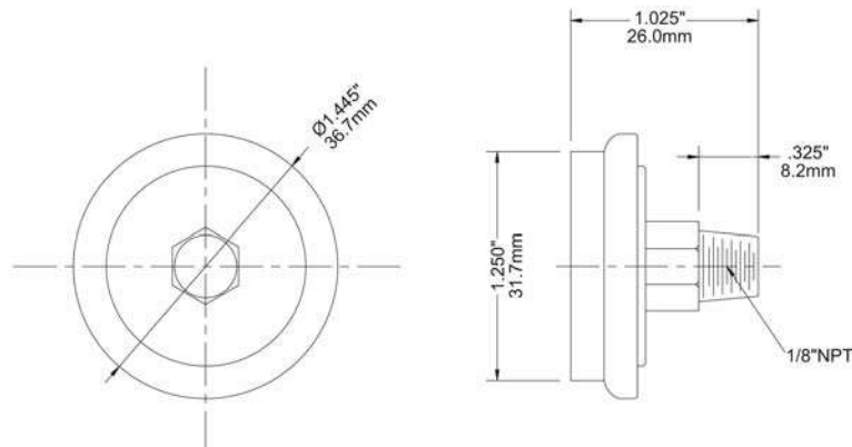
1.5" Spiral Tube Gauge
