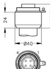
Buccaneer (IP 68) 7
