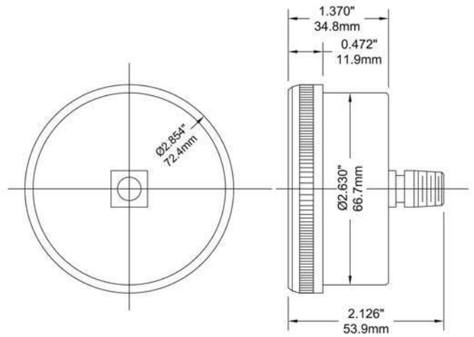
2.5" Back Connection
