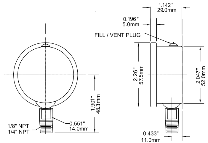
2" Bottom Connection
