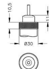
Cable outlet (IP 68) 5
