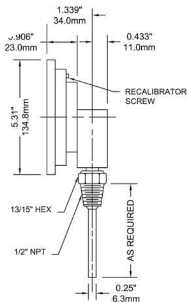
5" Bottom Connection
