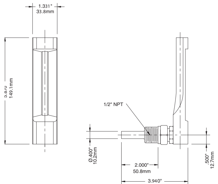
6" Angle
