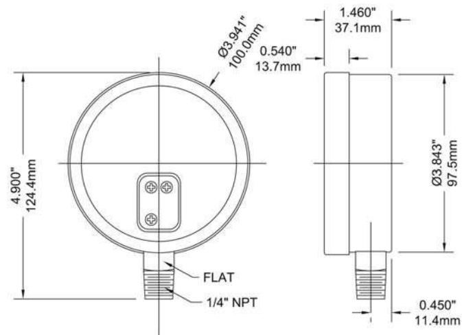
4" Bottom Connection
