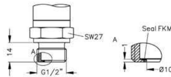
G1/2" semi-flush DIN 3852; M20x1.5 (up to 363 psi; nominal pressure abs. on request)
