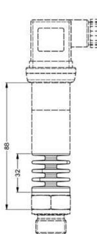
cooling element 300 °C 7
