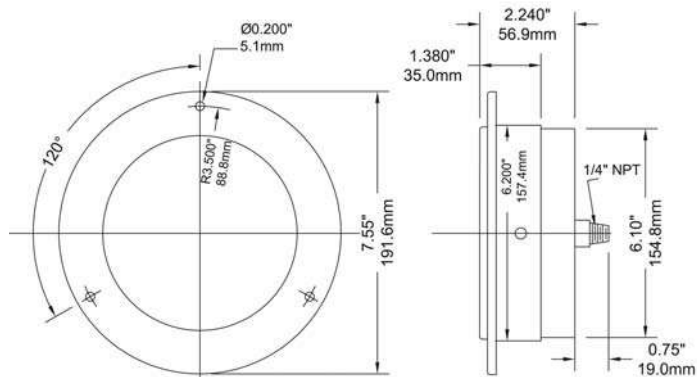
6" Back Connection Stainless Steel
