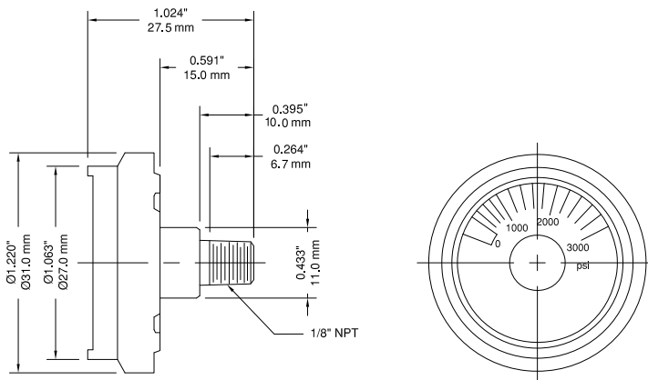
1.125" Spiral Tube Gauge
