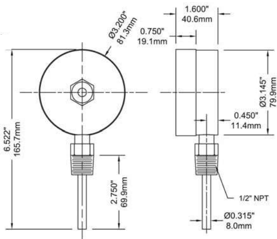
3" Bottom Connection
