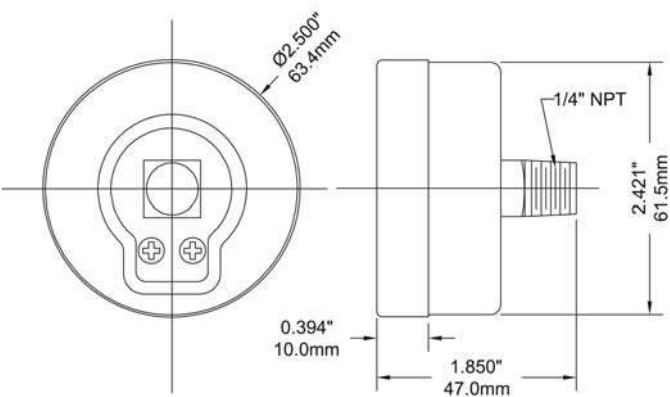
2.5" Back Connection
