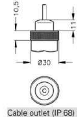
Cable outlet (IP 68)
