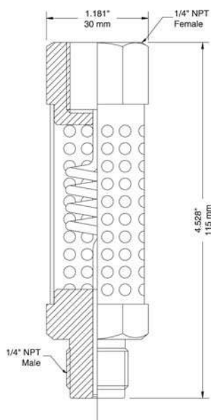
1/4" NPT Male x 1/4" NPT Female
