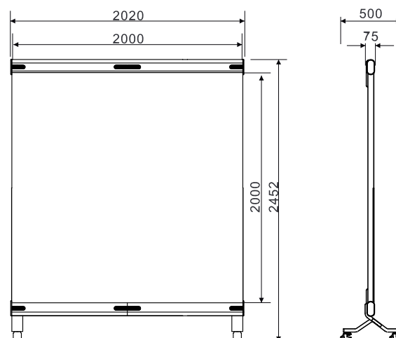
▼ External dimensions:2000*2000mm
