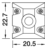
DIY Screw Connector DIY-SC-FR-15-D-01/02-DW
