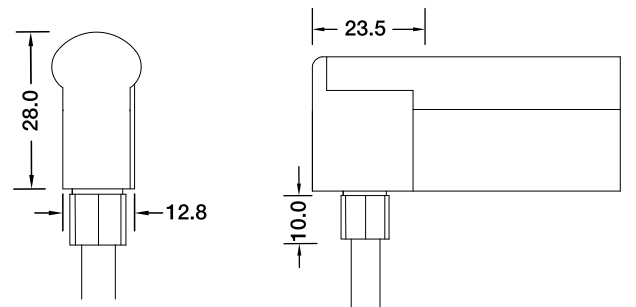
Bottom Entry Connector MJ-21-DW-B01/02/03 MJ-21-DW-B01SM MJ-21-DW-B02SF MJ-21-DW-B03SFM
