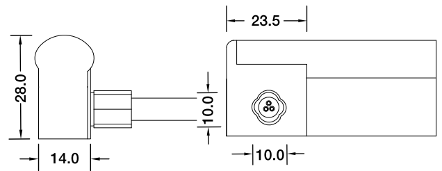
Side Entry Connector MJ-21-DW-S01/02/03 MJ-21-DW-S01SM MJ-21-DW-S02SF MJ-21-DW-S03SFM
