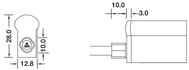
Direct Entry Connector MJ-21-DW-D01/02/03 MJ-21-DW-D01SM MJ-21-DW-D02SF MJ-21-DW-D03SFM
