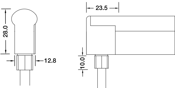
Bottom Entry Connector MJ-21-RGB-B01/02/03 MJ-21-RGB-B01SM MJ-21-RGB-B02SF MJ-21-RGB-B03SFM
