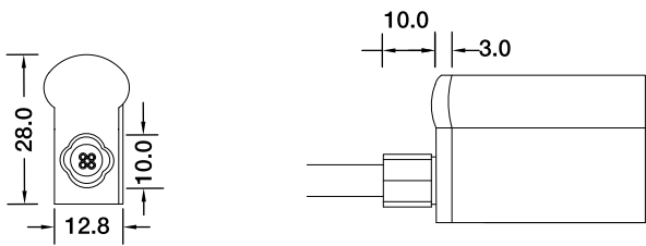
Direct Entry Connector MJ-21-RGB-D01/02/03 MJ-21-RGB-D01SM MJ-21-RGB-D02SF MJ-21-RGB-D03SFM
