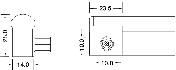
Side Entry Connector MJ-21-RGB-S01/02/03 MJ-21-RGB-S01SM MJ-21-RGB-S02SF MJ-21-RGB-S03SFM
