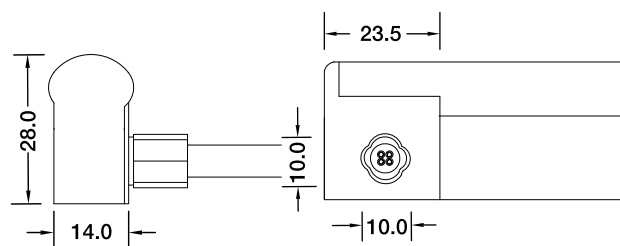
Side Entry Connector MJ-21-D4-S02SM MJ-21-D4-S03SFM
