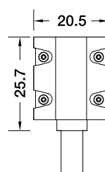
DIY Screw Connector DIY-SC-FR-15-B-01SF/02SM-D3
