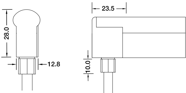
Bottom Entry Connector MJ-21-D3-B02SM MJ-21-D3-B03SFM
