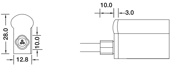
Direct Entry Connector MJ-21-D3-D02SM MJ-21-D3-D03SFM
