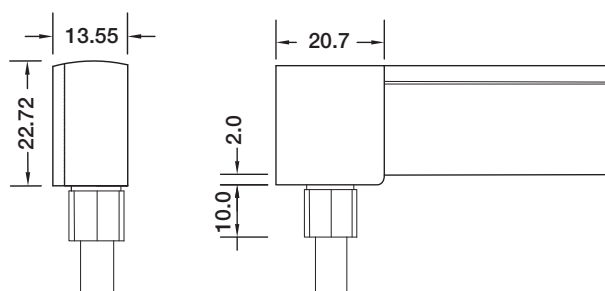
Bottom Entry Connector MJ-15-D4-S02SM MJ-15-D4-S03SFM
