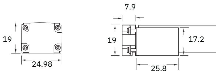
Male Connector SYZ-M12-M-5C-20AWG-D6-W-0327
