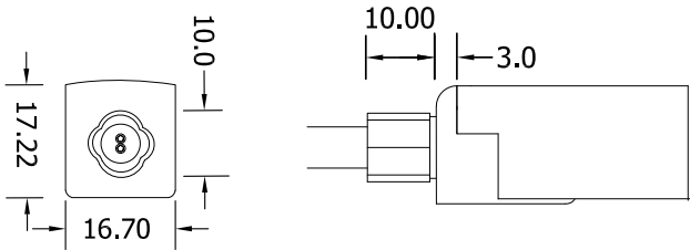
Direct Entry Connector MJ-17-A-D01/02/03 MJ-17-A-D01SM MJ-17-A-D02SF MJ-17-A-D03SFM
