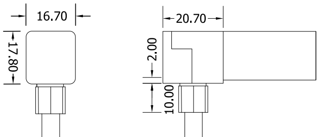
Bottom Entry Connector MJ-17-A-B01/02/03 MJ-17-A-B01SM MJ-17-A-B02SF MJ-17-A-B03SFM
