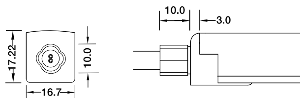
Direct Entry Connector MJ-18-A-D01/02/03 MJ-18-A-D01SM MJ-18-A-D02SF MJ-18-A-D03SFM
