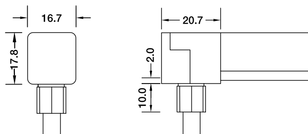
Bottom Entry Connector MJ-18-A-B01/02/03 MJ-18-A-B01SM MJ-18-A-B02SF MJ-18-A-B03SFM
