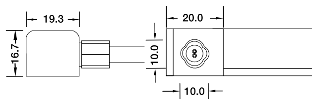
Side Entry Connector MJ-18-A-S01/02/03 MJ-18-A-S01SM MJ-18-A-S02SF MJ-18-A-S03SFM
