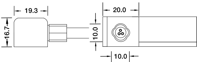
Side Entry Connector MJ-18-DW-S01/02/03 MJ-18-DW-S01SM MJ-18-DW-S02SF MJ-18-DW-S03SFM
