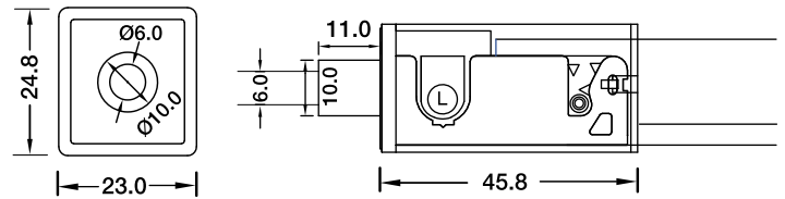
DIY Snap Connector DIY-SN-FR-16-D-01/02-D3
