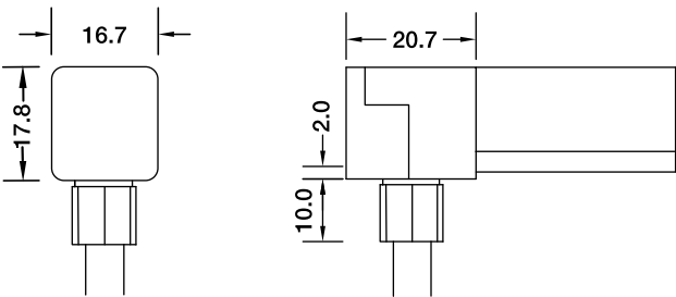
Bottom Entry Connector MJ-18-DW-B01/02/03 MJ-18-DW-B01SM MJ-18-DW-B02SF MJ-18-DW-B03SFM
