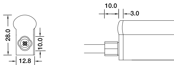
Direct Entry Connector MJ-SF21-RGB-D01/02/03 MJ-SF21-RGB-D01SM MJ-SF21-RGB-D02SF MJ-SF21-RGB-D03SFM
