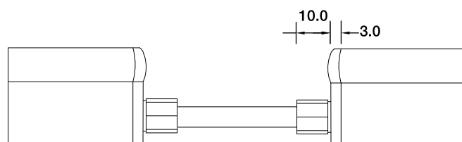
Jumper MJ-SF21-RGB-D-JC
