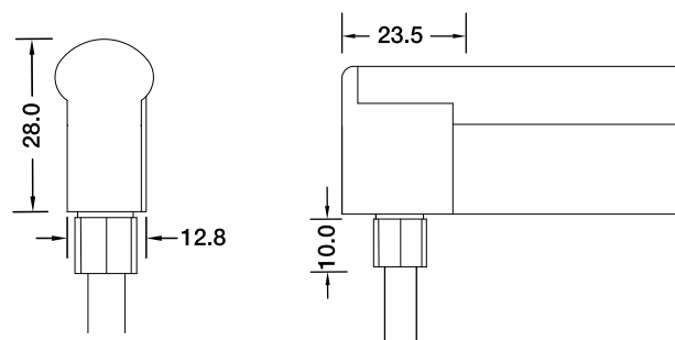
Bottom Entry Connector MJ-SF21-RGB-B01/02/03 MJ-SF21-RGB-B01SM MJ-SF21-RGB-B02SF MJ-SF21-RGB-B03SFM
