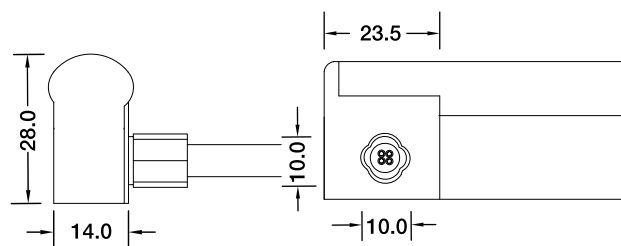
Side Entry Connector MJ-SF21-RGB-S01/02/03 MJ-SF21-RGB-S01SM MJ-SF21-RGB-S02SF MJ-SF21-RGB-S03SFM
