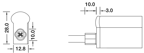
Direct Entry Connector MJ-SF21-RGBW-D01/02/03 MJ-SF21-RGBW-D01SM MJ-SF21-RGBW-D02SF MJ-SF21-RGBW-D03SFM
