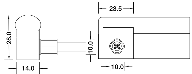
Side Entry Connector MJ-SF21-RGBW-S01/02/03 MJ-SF21-RGBW-S01SM MJ-SF21-RGBW-S02SF MJ-SF21-RGBW-S03SFM
