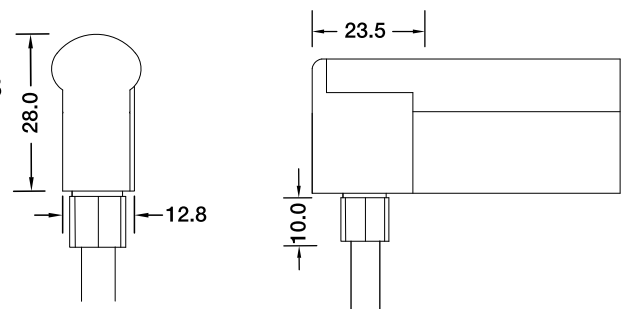
Bottom Entry Connector MJ-SF21-RGBW-B01/02/03 MJ-SF21-RGBW-B01SM MJ-SF21-RGBW-B02SF MJ-SF21-RGBW-B03SFM
